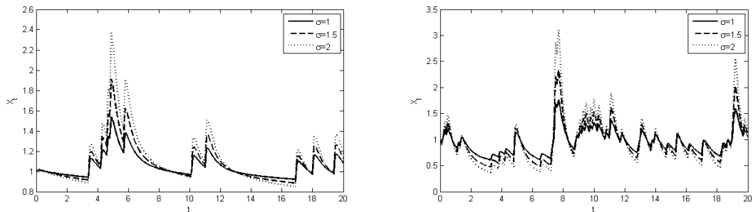
Figure 3: Sample paths of a solution of (5.6) for varying \sigma , fixed \lambda = 2.5 and d = 0.35 , using the same sample paths as in Figure 1, left \theta = 0.5 , right \theta = 2.5 .
