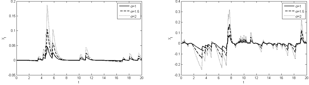
Figure 1: Sample paths of a solution of the Cox-Ingersoll-Ross model (5.3) with X_0 = 0 for varying \sigma , fixed \lambda = 2.5 and d = 0.35 , using two different FLP sample paths, left \theta = 0.5 , right \theta = 2.5 .
