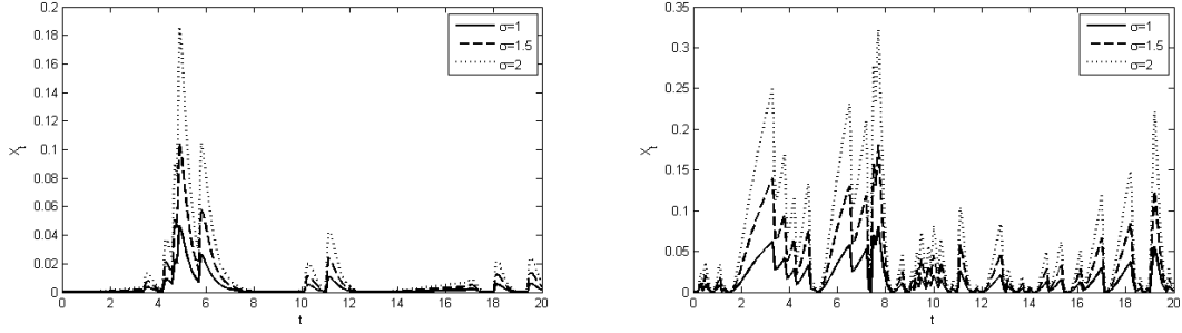
Figure 2: Sample paths of squared FLOUPs for varying \sigma , fixed \lambda = 2.5 and d = 0.35 , using the same sample paths as in Figure 1: left \theta = 0.5 , right \theta = 2.5 .
