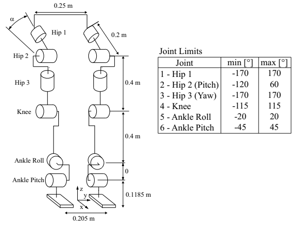
Fig. 3. Kinematic structure. The hip angle \alpha can be manually adjusted to 10, 20, and 30 degrees.
