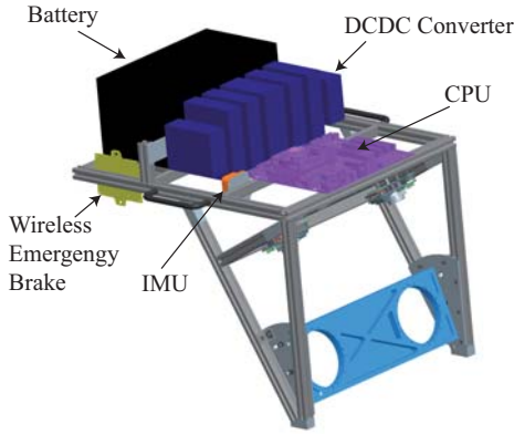
Fig. 8. Assembly in the trunk.
