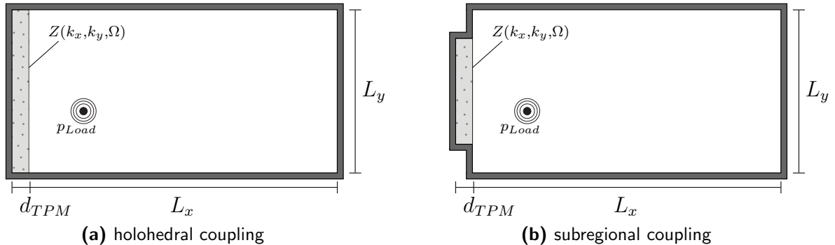
Figure 5.21: 2d structure with porous absorber
