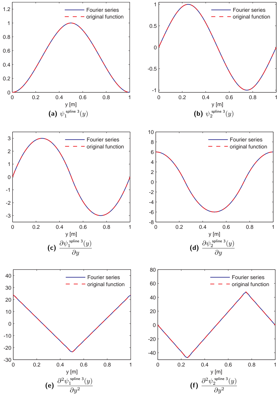
Figure A.5: Fourier approximation of the original trial function and its derivatives for a spline of order 3 \psi_{n_1}^{\text{spline } 3}(y) with r_{\max} = 15 Fourier members
