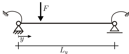
Figure 5.11: Euler-Bernoulli beam under a single load F
