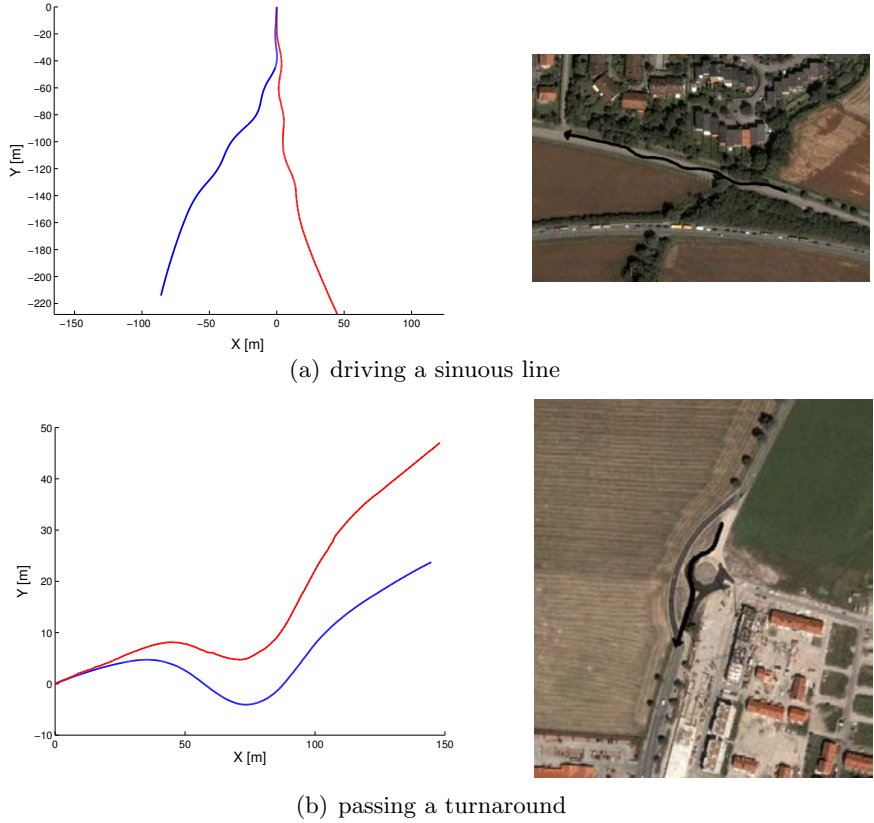
Figure 8.19: Two trajectories measured by the Z_\infty -algorithm (red) and an IMU (blue). In the pictures at the right-hand side the driven trajectories are sketched in black.
