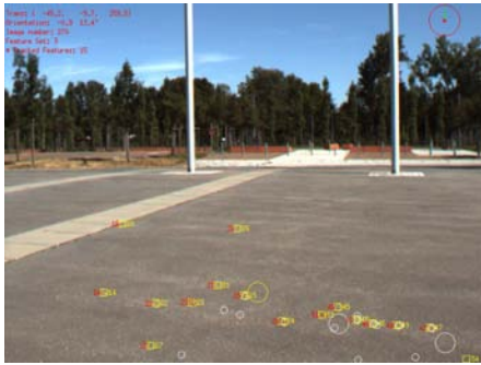
(a) VSLAM-screenshot
