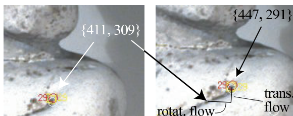
Figure 4.1: Two corresponding features in consecutive images acquired during high dynamic motions at a frame rate of 25 Hz. The feature drifts by 40.2 pixels, whereas 37 pixels result from rotation and 17 pixels from translation (some pixels cancel out). The red circle shows the feature propagation by the IMU and translation prediction in 2D. The yellow square illustrates the tracking result. The estimated location of the feature corresponds well enough to allow for local tracking.
