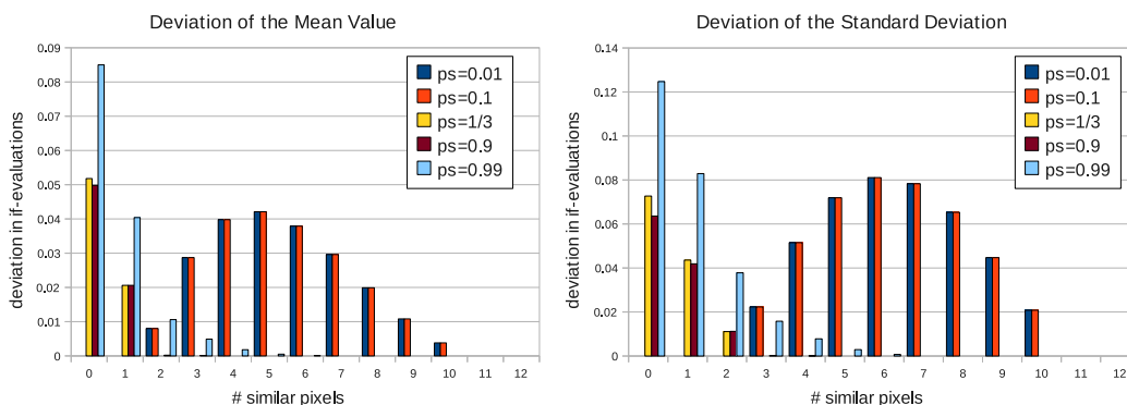
Figure 8.8: This chart illustrates the performance of various decision trees, based on different probabilities for a pixel to be similar ( p_s ). Each decision tree was tested with all possible pixel combination for the mask.
