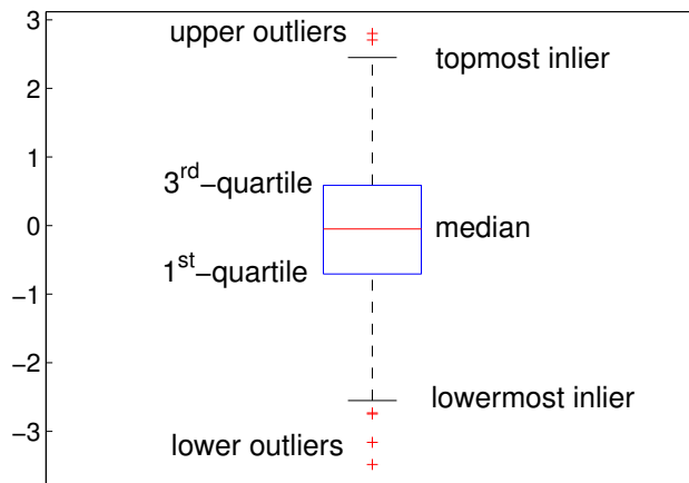
Figure A.1: A boxplot is a convenient way to illustrate the distribution characteristics of statistical population. The median, the 1 st - and 3 rd -quartile, the extend of the distribution and outliers are visualized by this representation. This plot has been generated by 1000 normal distributed random samples.
