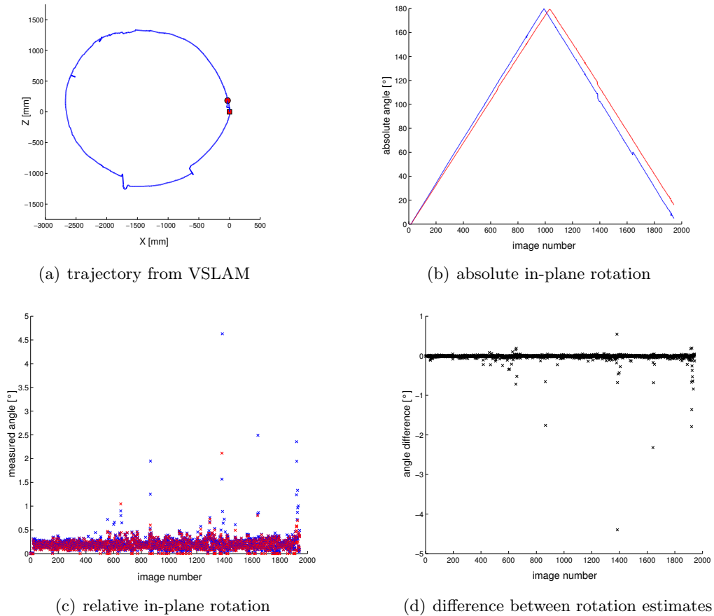
Figure 8.29: a) The computed trajectory by the VSLAM algorithm. The red square is the starting point and the red circle the endpoint of the path. b) Comparison of the absolute angle estimated by the Z_{\infty} (red) and the VSLAM (blue) algorithm. c) The relative angles about the Y-axis are plotted, which are computed by the Z_{\infty} - (red) and by the VSLAM-algorithm (blue). d) This plot shows the difference between the Z_{\infty} and VSLAM rotation estimates along the Y-axis. Only a few outlier can be identified, which are detected by the M-estimator in RVGPS. Hence, they have no effect on the final result.
