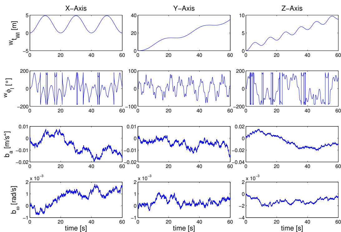
Figure 8.54: These plots denote the simulated motion for the filter experiments. We implemented an oscillating translational acceleration and rotational velocity, together with white Gaussian noise of the same magnitude as seen for real sensors.
