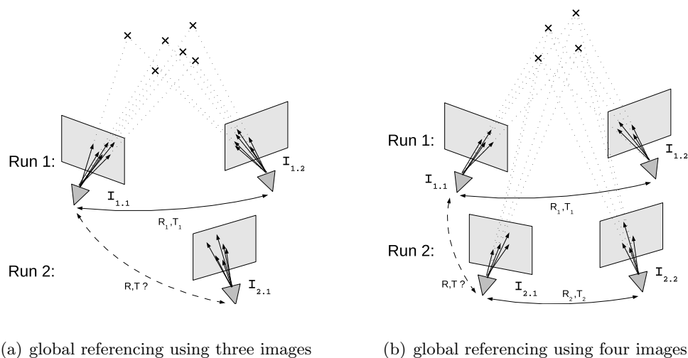
Figure A.2: These drawings sketch the principles of the 3- and the 4-images global referencing methods.
