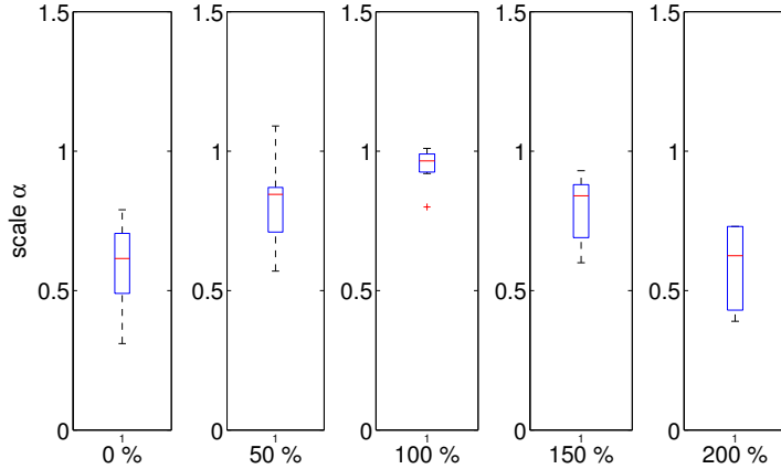
Figure 8.47: Estimated scale factor \alpha with respect to the temporal alignment: 0%, no temporal alignment; 100%, correct temporal alignment; 200%, twice the estimated delay between camera and IMU.
