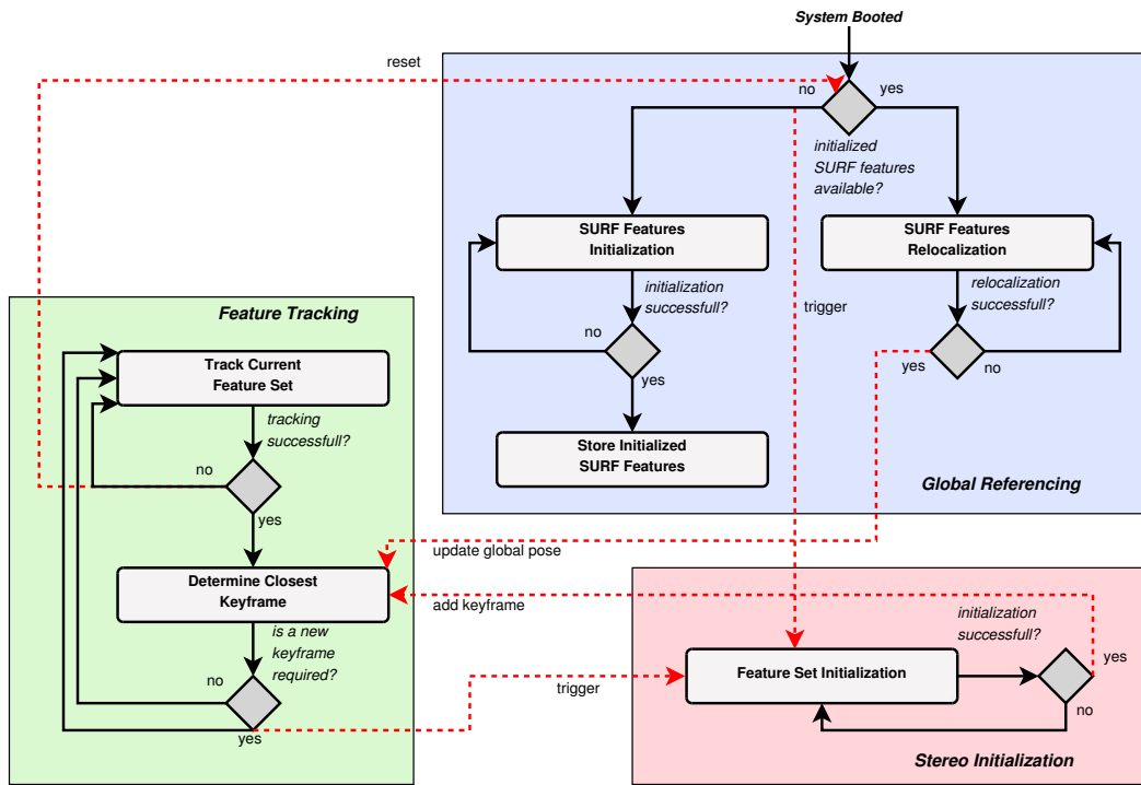
Figure A.4: The image-processing modules used for localization and global referencing. The synchronization triggers to ensure that the images of the different modules are synchronized are not illustrated for the sake of clarity.
