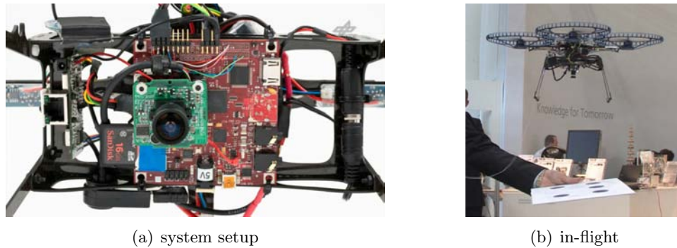
Figure 9.11: The left picture illustrates the bottom-view of the system setup, showing the Beagleboard and the Philips webcam. On the right hand side the quadcopter is shown while hovering fully autonomously above a hand-held board with the artificial markers printed on top.
