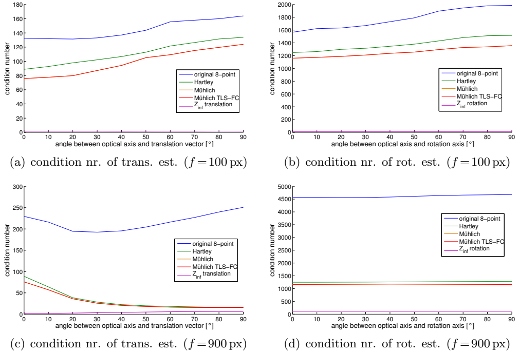
Figure 8.15: This plots compare the median condition numbers for the eight-point variants and the Z_{\infty} -algorithm. The left column shows the condition numbers for the translation estimation and the right one for the rotation estimation. The upper two plots were generated by simulating a wide angle camera ( f = 100 px) and the lower ones by a narrow field of view ( f = 900 px).
