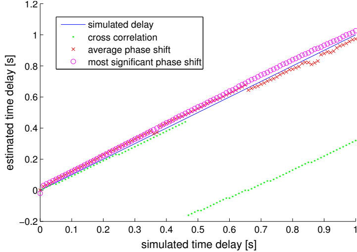
Figure 8.42: The blue line represents the simulated delay. The green dots are the correlation based results. The red crosses and the magenta circles are the average and the most significant phase shift output respectively.
