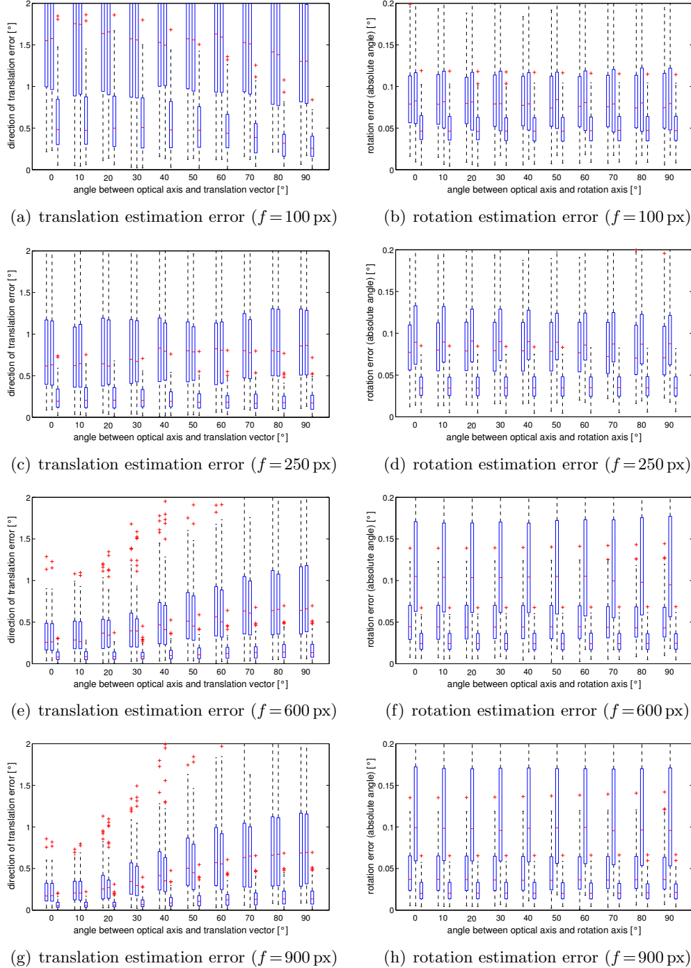
Figure 8.14: This graphic shows the error of translation and rotation estimation for various directions of translation and directions of rotation axis and different aperture angles (top to bottom: f = 100, 250, 600 and 900 px). Following algorithms are compared (from left to right): the eight-point algorithm (original and Mühlich variant) and the Z_\infty -algorithm. Some boxplots of the eight-point algorithm might be cropped for the sake of visibility of the Z_\infty -boxplots. However, the full boxplots are shown in Fig. 8.10 to Fig. 8.13.
