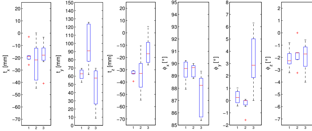
Figure 8.49: Estimation of {}^I\mathbf{t}_{IC} and the Euler angles {}^I\boldsymbol{\phi}_C corresponding to {}^I\mathbf{q}_C (boxplots). 1-left: B-spline, 2-middle: grey box, 3-right: UKF.
