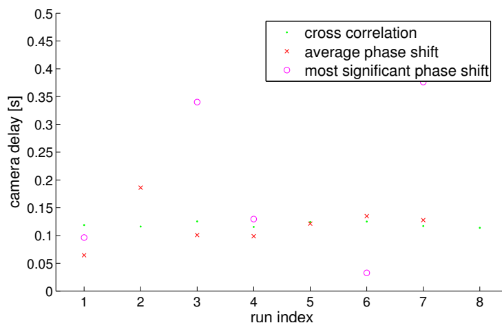
Figure 8.43: The cross-correlation reliably estimates the time delay, while the phase congruency methods are not as robust. Some of their estimates are not even visible because of the scaling which has been chosen for the sake of detail.
