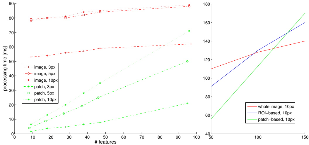
Figure 8.1: These figures compare the processing times of the KLT-variants for different number of features to track. The red values represent the whole-image-based implementation, the blue values the ROI-based version and green are the times for the patch-based variant. On the left, different sizes for the search window are chosen. While the processing time for the whole image almost only depends on the number of pyramid layers (3 px search range results in one, 5 px and 10 px in two pyramid layers), the patch-based approach is also related to the search range and the number of features. The right image shows the intersection of the lines for a 10 px search range.
