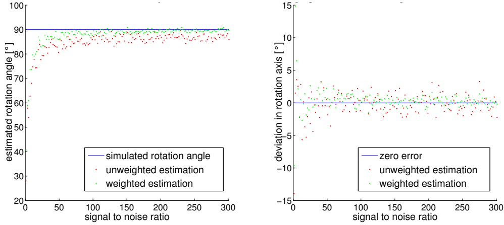
Figure 8.44: The left image shows the results for the absolute rotation angle, the right picture illustrates the angular error between the estimated and simulated rotation axis. The blue line represents the simulated absolute angle and the zero-error line respectively. By increasing the signal to noise ratio the performance of both, the weighted (green) and the unweighted (red) rotation estimation, increases.
