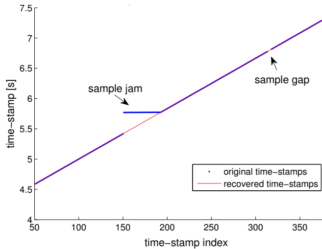
Figure 8.39: The blue dots represent the time-stamps of a clipped image sequence. The red line shows the fixed-time line without data jams and gaps.
