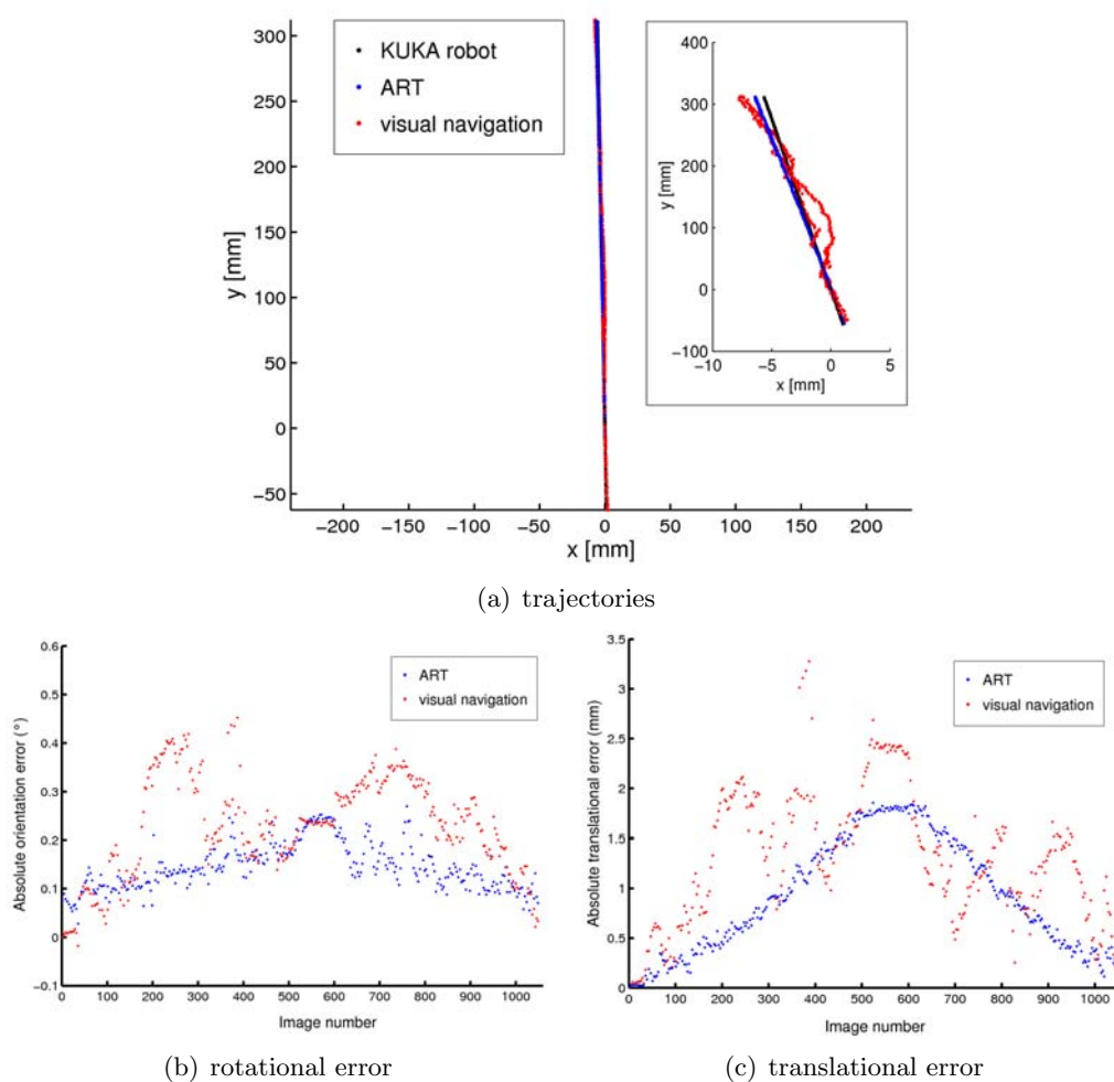
Figure 9.6: a) The scan trajectories computed by three different references. By zooming in the x-axis (small plot) the error becomes evident. The absolute rotational error ( b) and the absolute translational error ( c) are referenced to the KUKA poses.
