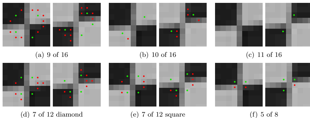
Figure 8.6: The corner response for different AST pattern. Detected features are colored in red. The corners after non-maximum suppression are green.
