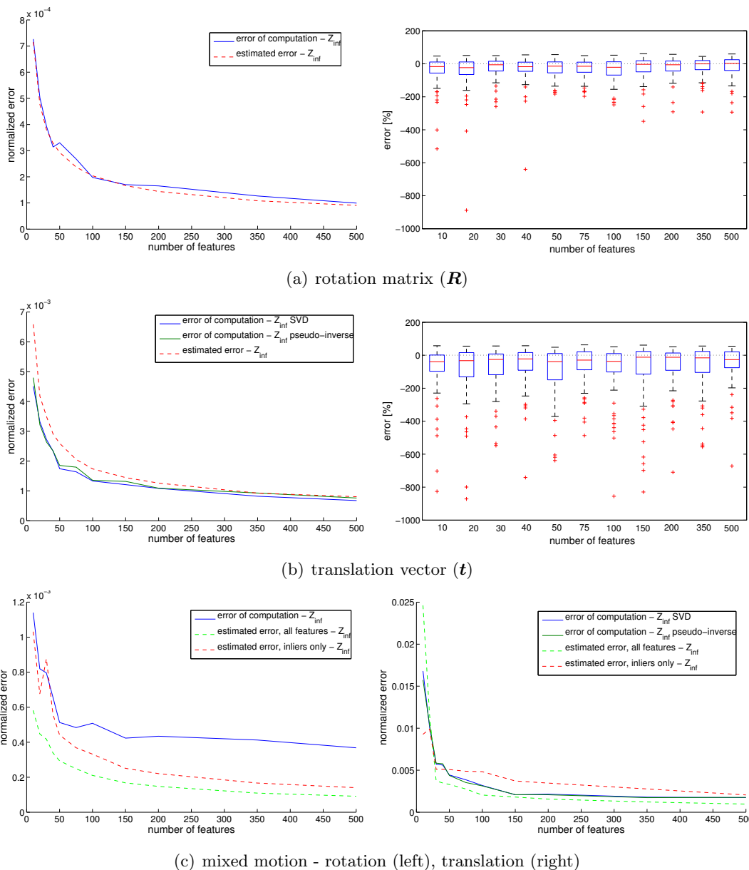
Figure 8.36: This graphic shows on the upper two left plots the median error of the computed and the simulated rotation matrix \mathbf{R} and translation vector \mathbf{t} for a varying number of features. On the right hand side the corresponding relative errors of the error-propagation are illustrated as boxplots. The lower two images show the performance if both motions, rotation and translation, are simulated and estimated at the same time. The simulated camera parameters are: noise in both images due to pixel-discretization of the features ( \sigma^2 = \frac{1}{12} ), 600 \times 600 pixel resolution and 250 px focal length ( \approx 100^\circ aperture angle).
