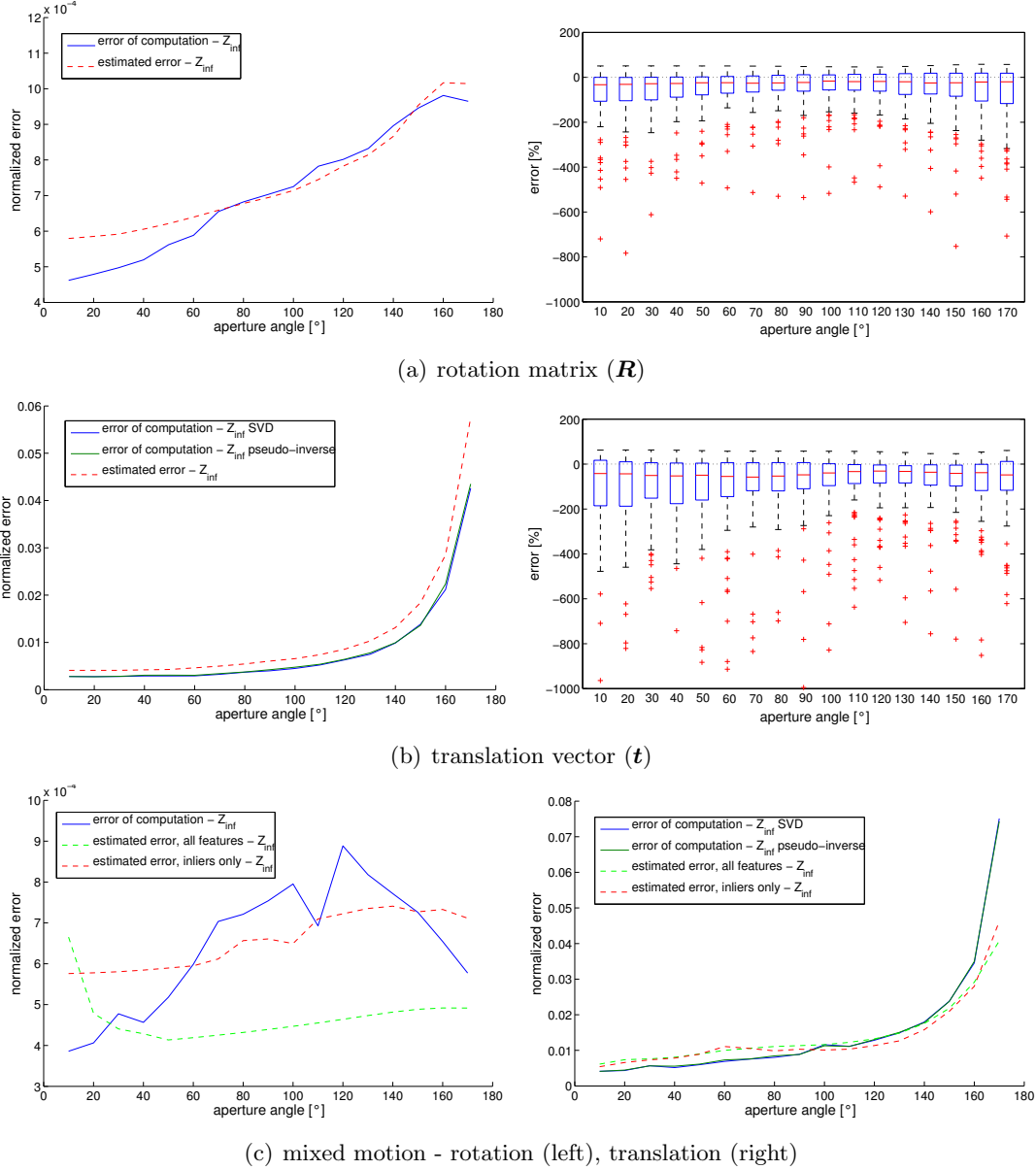
Figure 8.35: This graphic shows on the upper two left plots the median error of the computed and the simulated rotation matrix \mathbf{R} and translation vector \mathbf{t} for different aperture angles. On the right hand side the corresponding relative errors of the error-propagation are illustrated as boxplots. The lower two images show the performance if both motions, rotation and translation, are simulated and estimated at the same time. The simulated camera parameters are: 10 or 20 features depending on whether only one motion component (rotation or translation) or both components are simulated, noise in both images due to pixel-discretization of the features ( \sigma^2 = \frac{1}{12} ) and 600 \times 600 pixel resolution.
