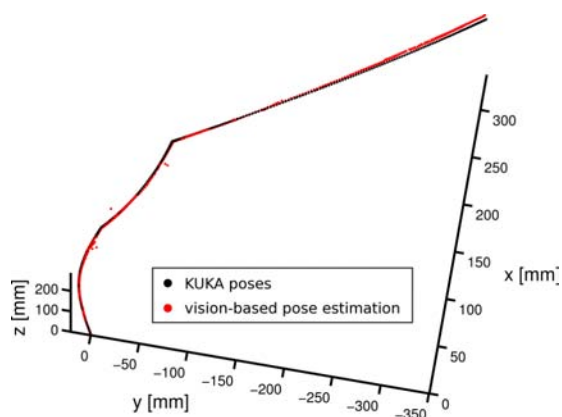
Figure 8.25: This figure shows the executed trajectory and compares the result of the keyframe-based SLAM (red) with the inverse-kinematics of the KUKA robot (black).
