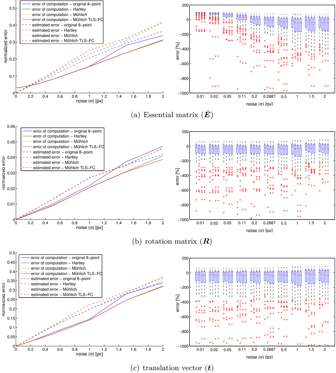
Figure 8.33: This graphic shows on the left hand side the median error of the computed and the simulated Essential matrix \bar{\mathbf{E}} , rotation matrix \mathbf{R} and translation vector \mathbf{t} for different noise levels and for all four introduced eight-point implementation variants. On the right hand side the relative errors of the uncertainty-propagation are illustrated as boxplots. The same noise is simulated in both images. The value 0.2887 denotes noise by pixel-discretization as assumed for the former plots. The simulated camera parameters are: 10 features, 600 \times 600 pixel resolution and 250 pixel focal length ( \sim 100^\circ aperture angle).
