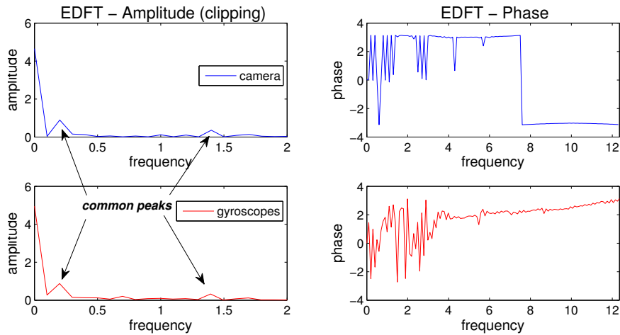
Figure 8.41: This figures illustrate the phase shift based temporal alignment for the simulated data. The left images show the amplitude and the right the phase spectrum of the gyroscope (red) and camera (blue) data.
