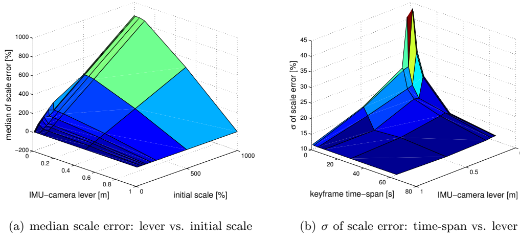
Figure 8.58: The left plot illustrates the relation between IMU-camera lever and the quality of the scale initialization. It shows, that a large lever can compensate for a bad initialization. The right plot illustrates the standard deviation of the scale estimation for a different time-span between keyframes and changing IMU-camera lever sizes. It confirms that a large lever size leads to a much quicker scale convergence than a short one.
