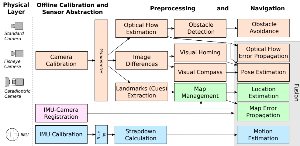
Figure 1.3: This flow diagram illustrates significant software modules for an efficient autonomous robot system which is based on a camera (red) and an IMU (blue). Basically all tasks can be achieved by processing the camera measurements only. Whereas, the IMU increases accuracy and robustness especially at high dynamics, and the systems reliability, because it is a fail-safe sensor which does not depend on the environment. The navigation map can be based on arbitrary sensors and, thus, these modules are colored in green.
