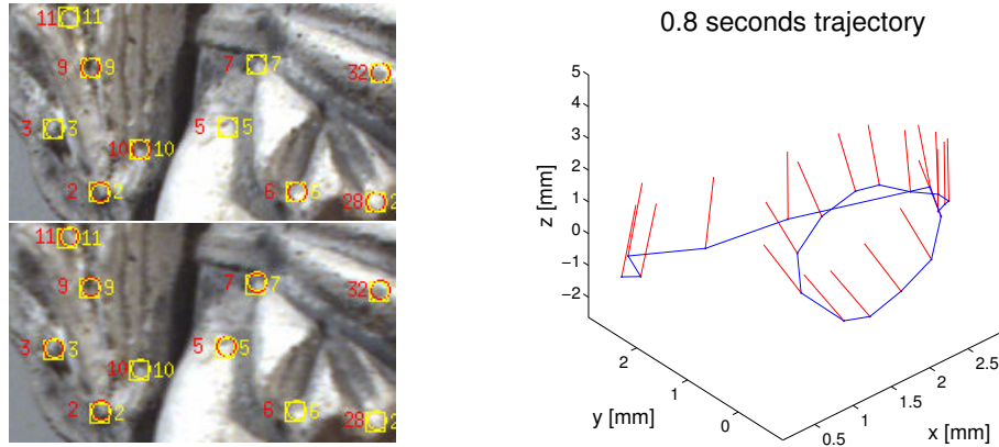
Figure 8.53: The left two images show two screenshots acquired at the beginning and at the end of a fast camera motion (up to 14^\circ per frame). The yellow squares mark the IMU-supported propagation of the landmarks, while the red circles are the tracked features. The yellow circles are the reprojection of the features according to the 3D structure. The right picture illustrates the trajectory (blue) and the camera viewing directions (red).
