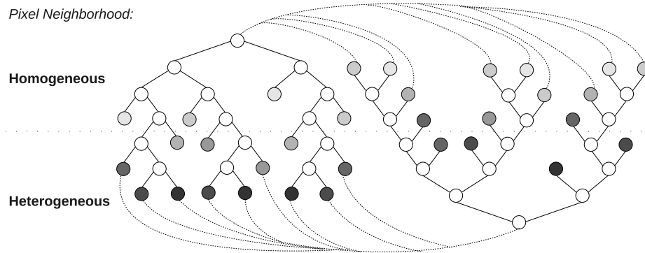
Figure 7.1: Principle of the adaptive and generic accelerated segment test. The AGAST switches between two (or more) specialized trees as soon as the pixel neighborhood changes. The lighter the gray of a leaf the more equal pixels are in the configuration. The left tree achieves less pixel evaluations (shorter decision paths) in a homogeneous pixel neighborhood, while the right one is optimized for textured regions.
