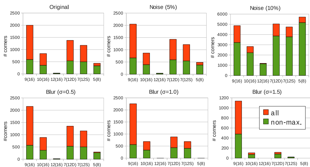
Figure 8.7: These charts compare the corner response of different patterns for blurry and noisy images. To preserve the comparability we use the arc length S and in brackets the mask size for labeling. The red bars show the total amount of features found, while the green bars represent the number of corners after non-maximum suppression. Note that the scales of the charts are not the same.
