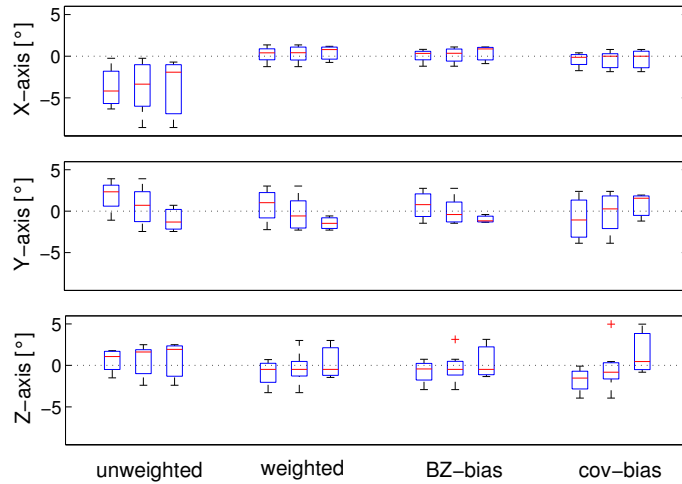
Figure 8.45: These box plots show the performance of the presented rotational alignment methods. Therefore, the estimated Euler angles between IMU and camera have been subtracted from a “ground truth” estimate gathered by a brute force search with resolution 0.5^\circ . The leftmost box plot of each set corresponds to the four short runs, the rightmost to three of the long runs and the center box plot represents all seven runs.
