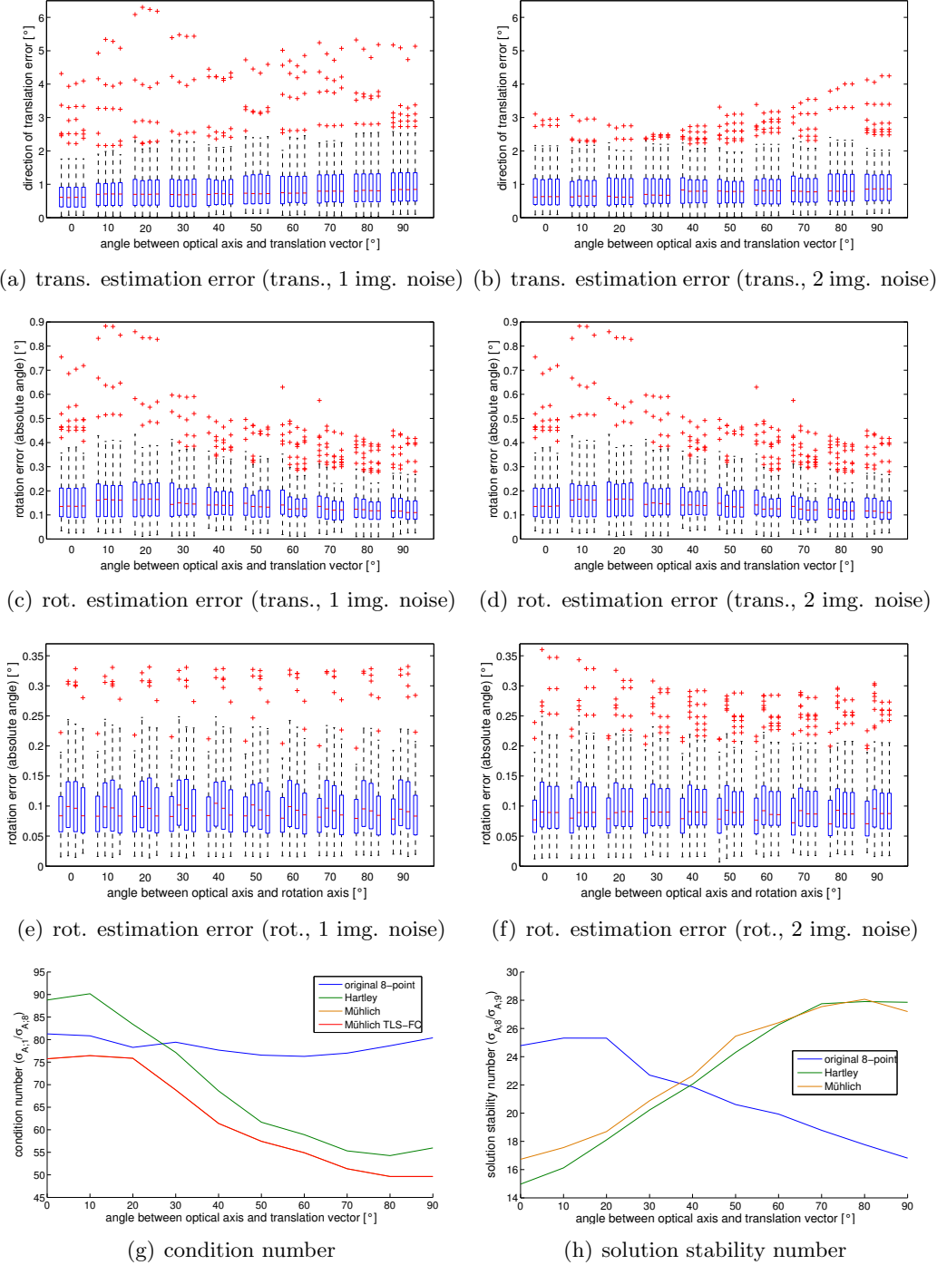
Figure 8.11: This graphic shows the error of translation and rotation estimation of the eight-point algorithm for different directions of translation and of the rotation axis simulating a focal length of 250 px, which is equivalent to an aperture angle of \sim 100^\circ . The lower two plots illustrate the condition and stability number as described in the text. The simulation parameters used are: 10 features, noise in both images due to pixel-discretization of the features ( \sigma^2 = \frac{1}{12} ) and 600 \times 600 pixel resolution.
