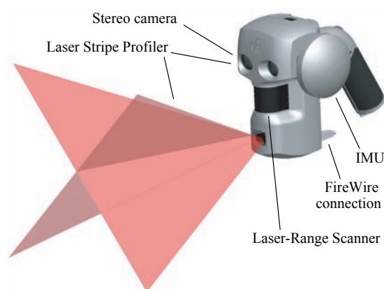
Figure 9.1: The major sensors of the DLR 3D-Modeler are the stereo cameras, the LSP, the LRS and an IMU.
