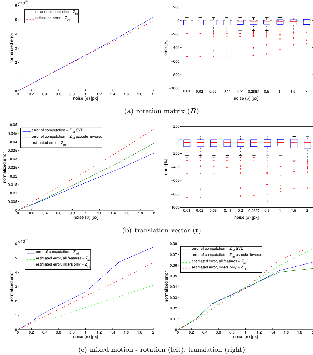
Figure 8.37: This graphic shows on the upper two left plots the median error of the computed and the simulated rotation matrix \mathbf{R} and translation vector \mathbf{t} for various levels of noise. On the right hand side the corresponding relative errors of the error-propagation are illustrated as boxplots. The lower two images show the performance if both motions, rotation and translation, are simulated and estimated at the same time. The simulated camera parameters are: 10 or 20 features depending on whether only one motion component (rotation or translation) or both components are simulated, 600 \times 600 pixel resolution and 250 px focal length ( \approx 100^\circ aperture angle).
