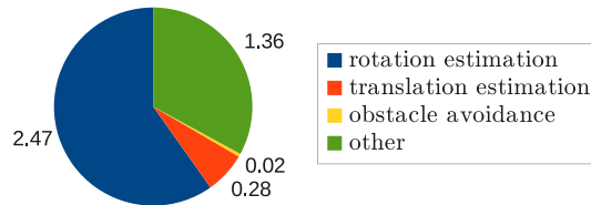
Figure 8.23: The computation time for each module of the Z_\infty -algorithm in milliseconds.
