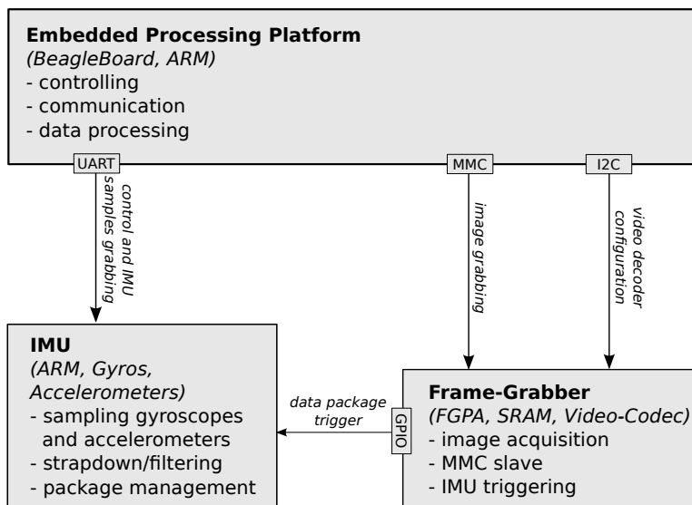
Figure A.5: This graphic illustrates the components of the hardware-synchronized IMU-camera setup. The IMU generates image specific inertial measurement bundles, triggered by the vertical synchronization signal of the camera.
