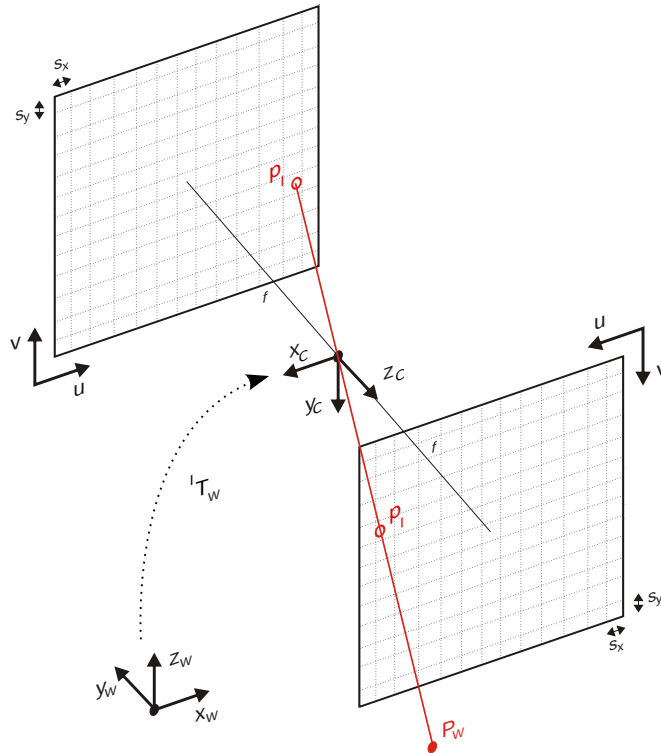
Figure 2.1: This drawing illustrates the camera projection with the intrinsic and extrinsic camera parameters. While the real image plane is behind the optical center (the pinhole, the point through which all the rays go), it is usually easier for imagination to assume a plane which is in front of the optical center. In this plane all the objects are upright and not mirrored as in the real image plane.
