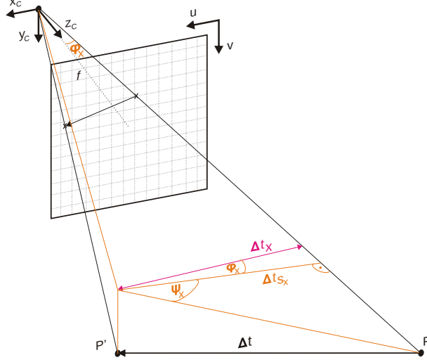
Figure 5.2: This drawing visualizes how the measurable translational component \Delta t_x can be calculated. In general the optical flow vectors become longer the more parallel the translation to the image plane is and the closer the features are to the image border (due to a higher angular resolution). The orange auxiliary line illustrates the projections onto the X-Z plane.
