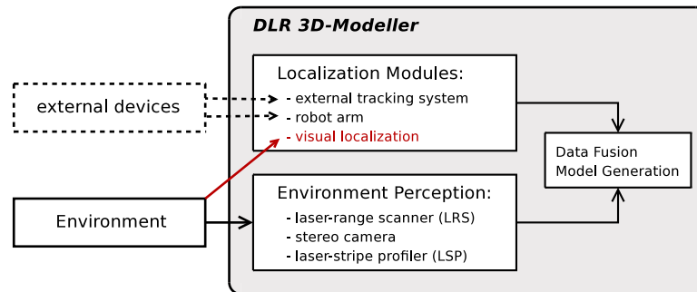
Figure 9.2: This figure illustrates the modules provided within the DLR 3D-Modeler. Due to the visual localization module, there is no external device necessary anymore.
