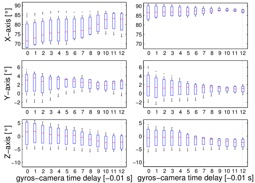
Figure 8.46: These boxplots show the performance of the unweighted and weighted rotation estimation on not correctly temporally aligned real data. The black dotted line corresponds to the mean of the estimated delays between camera and gyros of all runs.
