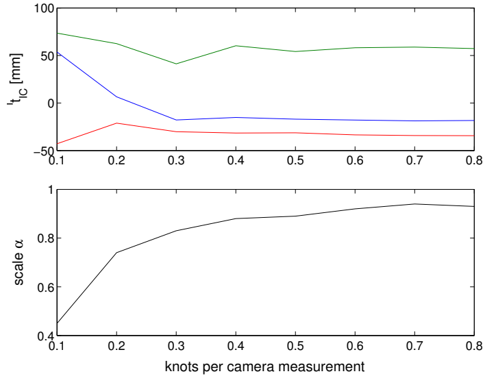
Figure 8.51: Estimated relative pose {}^I t_{IC} (above) and scale \alpha (below) with respect to the number of knots.
