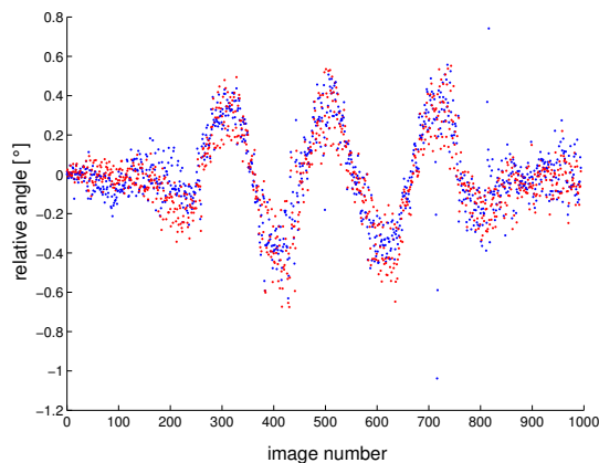
Figure 8.20: This image shows the relative angle measured during the same run as in the left image of Fig. 8.19. The Z_\infty -rotation estimation is red, while the IMU data is blue.
