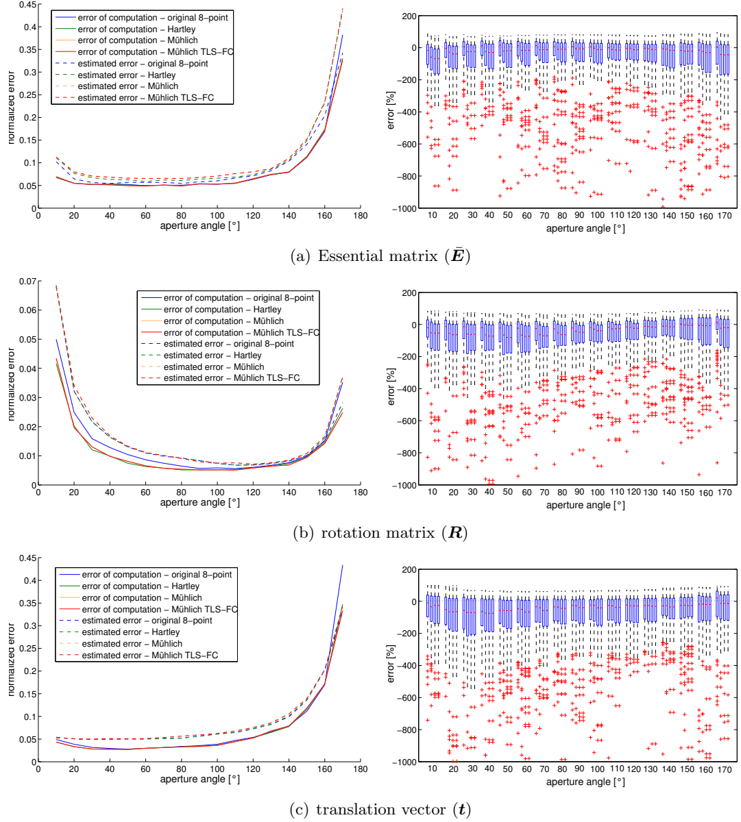
Figure 8.31: This graphic shows on the left hand side the median error of the computed and the simulated Essential matrix \bar{\mathbf{E}} , rotation matrix \mathbf{R} and translation vector \mathbf{t} for different aperture angles and for all four introduced eight-point implementation variants. On the right hand side the relative errors of the uncertainty-propagation are illustrated as boxplots. The simulated camera parameters are: 10 features, noise in both images due to pixel-discretization of the features ( \sigma^2 = \frac{1}{12} ) and 600 \times 600 pixel resolution.
