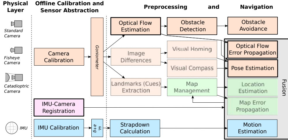
Figure 10.1: In this figure, we illustrate again the flow diagram which we proposed in the motivation and already depicted in Fig. 1.3. However, this time we highlight the modules for which we presented contributions in this thesis and greyed out the ones which are in the focus of future work. At this point we are able to provide efficient inertial-visual odometry. The next major steps consist in providing a sort of topological map as global reference and implementing efficient homing algorithms.
