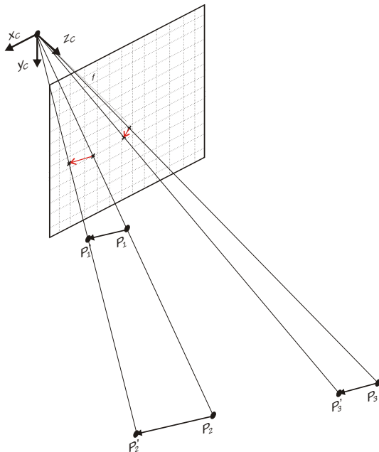
Figure 5.1: Optical flow vector 1 ( P_1, P_1' ) is shorter than vector 2 but it is closer to the optical center. Therefore, both vectors result in the same projection. Vector 3 has the same length as vector 1, but it is farther from the image plane, hence, the projection is much shorter. It is so small, that the projection of P_3 and P_3' lies within the same pixel. If such a projection results only from a translation then this feature would be translation-invariant, because the translation does not yield a measurable motion.
