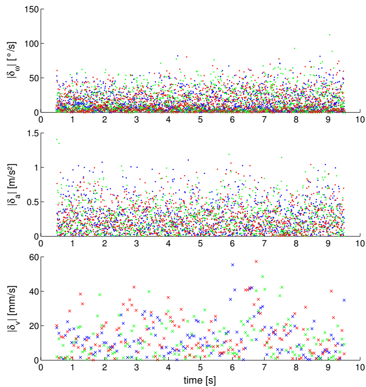
Figure 8.48: Error between the simulated measurements and the estimated trajectories. Please note that the crosses represent the camera measurements which are closer to zero due to less noise assumed for the camera. The upper plot illustrates both angular velocities \omega^I and \omega^C , the middle plot shows a^I and the lower one v^C . The errors of the estimation correspond to the simulated noises.
