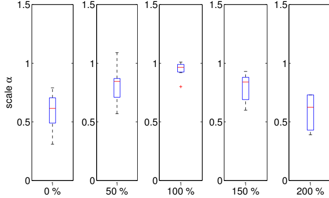
Figure 8.52: Estimated scale factor \alpha with respect to the temporal alignment: 0%, no temporal alignment; 100%, correct temporal alignment; 200%, twice the estimated delay between camera and IMU.
