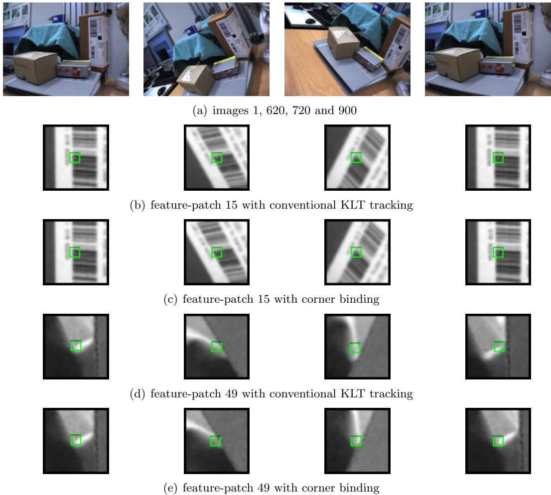
Figure 8.2: Two different patches are tracked in an image sequence with and without corner binding. Fig. 8.2(a) shows the images where the features are extracted. While patch 15 differs only by one pixel from the original location after 900 tracking steps, patch 49 has been drifted much further due to partially occlusion. For these two patch-sequences, the corner-binding variant nullifies the accumulated tracking residues. The green square illustrates the integral-window and the green point its center and, thus, the feature location.
