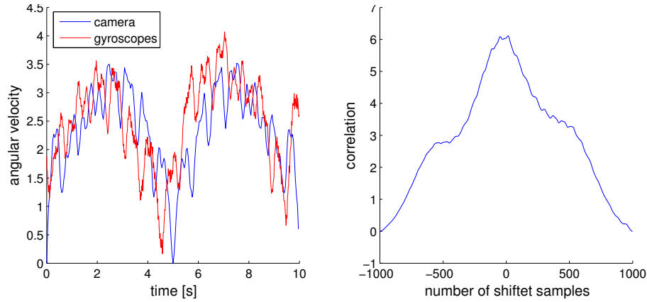
Figure 8.40: The left figure illustrates the unaligned simulated gyroscope (red) and camera data (blue), while the right figure shows the cross correlation of the data.
