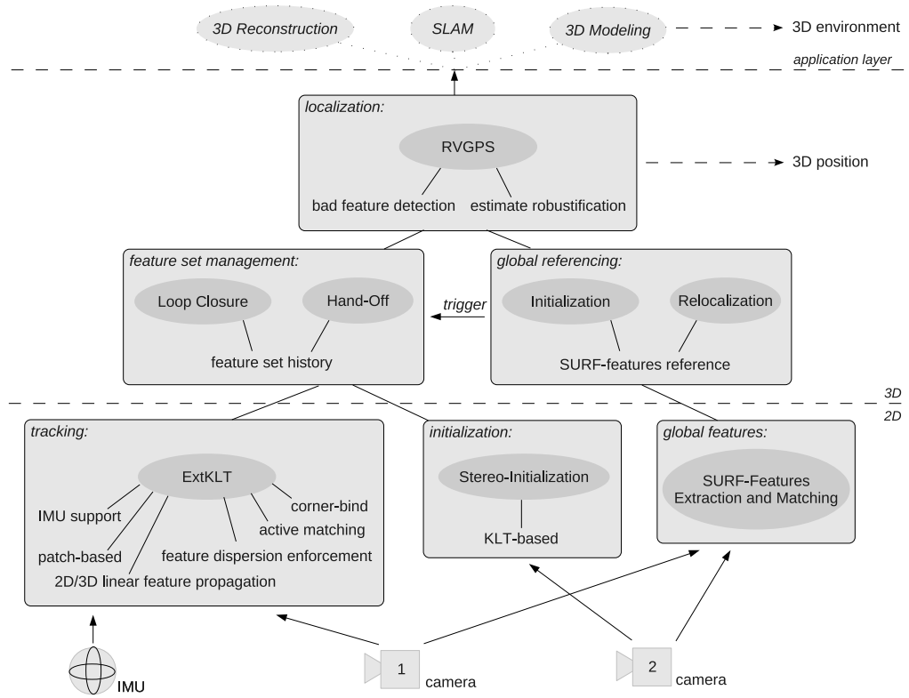
Figure 9.4: This block diagram illustrates the modules, which are used for the image-based localization.
