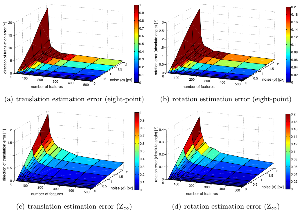
Figure 8.17: This graphic plots the influence of the detection accuracy and the number of features against each other. The eight-point algorithm used is the Mühlich-variant. The simulation parameters are: noise in both images, 600 \times 600 pixel resolution and 250 px focal length ( \sim 100^\circ aperture angle).
