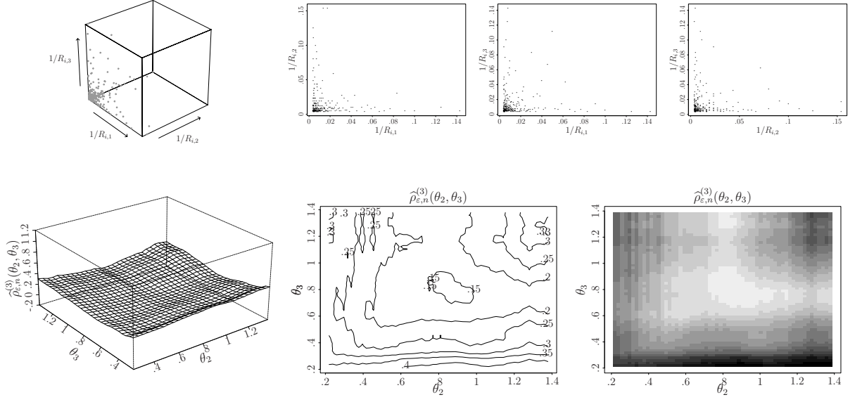
Figure 7: First row: data (3-d and 2-d projections) of the ranks 1/R_{i,j} , 1 \leq j \leq 3 , of the low dependent 7-day swap rates in USD, EUR and GBP.
