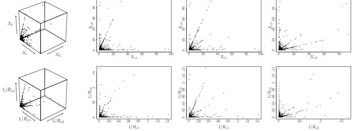
Figure 3: First row: data (3-d and 2-d projections) of the model given in Example 5.2. Second row: ranks 1/R_{i,j} , 1 \leq j \leq 3 , in the same order as in row one.
