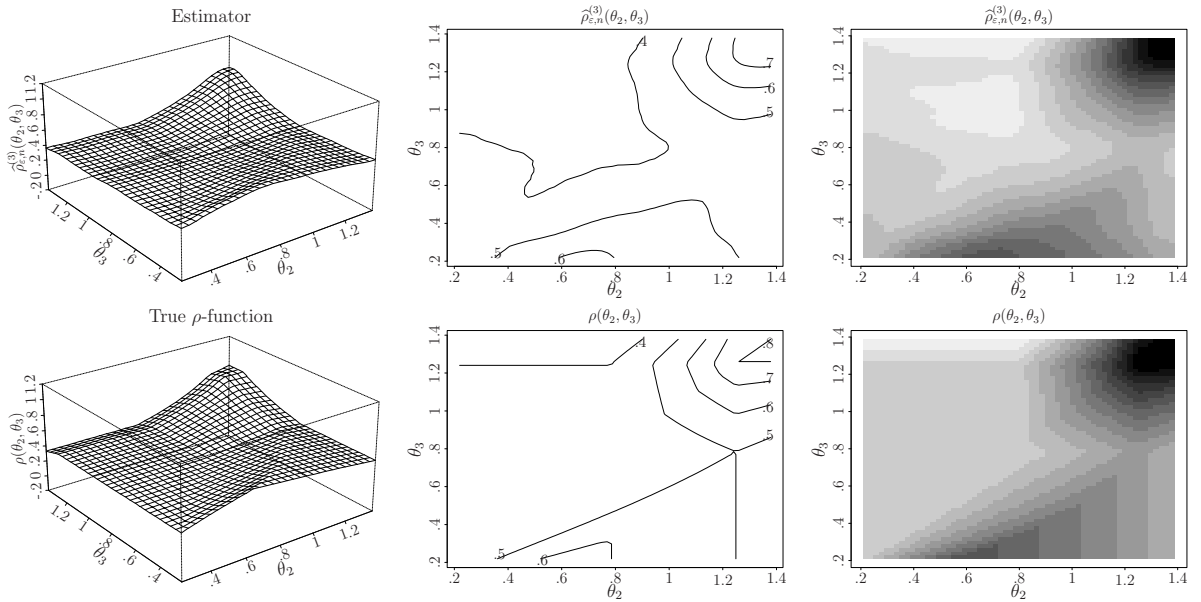
Figure 4: First row: smoothed estimate \widehat{\rho}_{\varepsilon,n}^{(3)}(\theta_2, \theta_3) of the simulated data (see Figure 3), with perspective plot (left-most), contour plot (middle) and image plot (right-most). Second row: true tail dependence function \rho(\theta_2, \theta_3) for this model.
