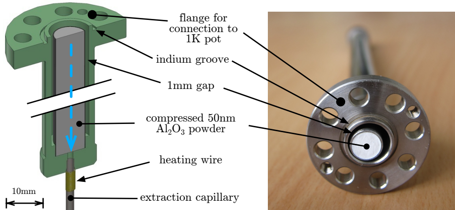
Figure 2.7: Technical drawing ( left ) and photograph ( right ) of the superleak in SUN2. The blue dotted line (—) indicates the direction of the extracted superfluid in to the production volume. The total length of the superleak is \approx 17 cm, for scale.
