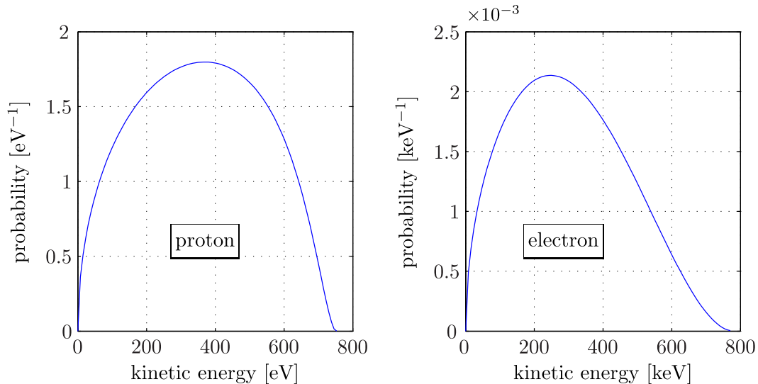
Figure 7.1: The energy spectrum of the protons and electrons produced from neutron \beta -decay. The expressions for the spectra are taken from Ref. [Sim10]. The electron antineutrino angular correlation a = -0.103 (the present world average) in the former; and the Fermi function F(E) = 1 in the latter.
