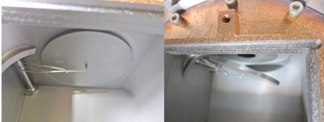
Figure 3.4: Left: The UCN flap valve in the closed position, as seen from the direction of the CN beam with the long aluminium inner UCN production volume removed. The beryllium plate, stainless steel wiring and stainless steel axle is visible. Right: The UCN flap valve opened, viewed from a similar angle as before. The bottom of the stainless steel conical piece can be seen. The copper transition plate used to fix the rectangular aluminium inner production volume to the circular copper end piece can also be seen. The opening angle of the UCN flap valve shown is just an example and does not reflect the actual angle used in the experiments. For scale, the beryllium plate is 61 mm in diameter and 3 mm thick.
