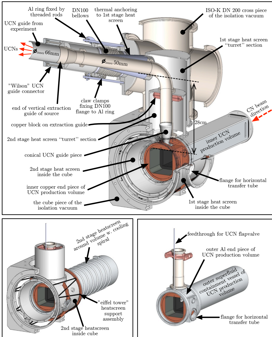
Figure 3.1: The prototype UCN production tower used in the PF1b experiment. Not shown are the flanges of the DN200 cross piece and cube, and the back flanges and foils of the UCN production volume and heat screens (shown in Fig. 3.7). Top : Certain sections cut out to reveal the UCN extraction system and the inner UCN production volume. The end aluminium piece of the UCN production volume is shown as a black transparent frame only. Bottom-left : Only the 2nd stage heat screens are shown so that the “eiffel tower” can be seen. Bottom-right : The containment vessel of the UCN production volume.
