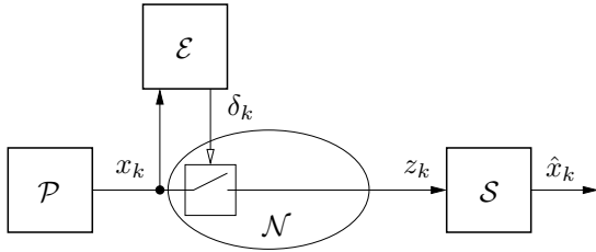
Figure 1: System model of the networked control system with plant \mathcal{P} , event-trigger \mathcal{E} , state estimator \mathcal{S} and communication channel \mathcal{N} .
