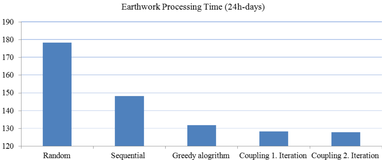
Figure 6: Comparison of earthwork processing times using different approaches
