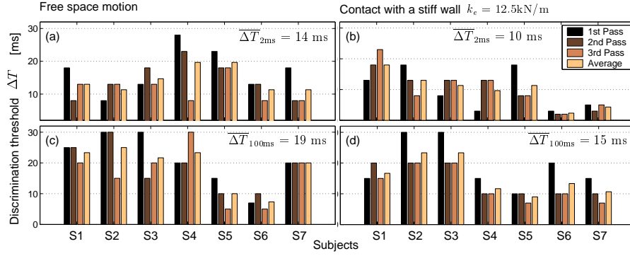
Fig. 9. Results of human user study: discrimination thresholds for time delay \Delta T at reference time delays T_0 = 2 ms (a), (b) and T_0 = 100 ms (c), (d) for free space motion (a), (c) and contact with a stiff wall (b), (d).
