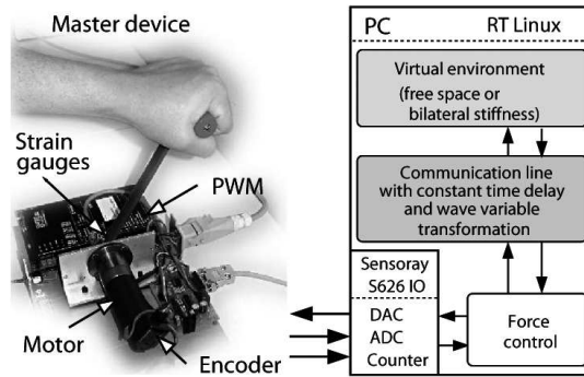
Fig. 7. Experimental system architecture with a 1DoF telerobotic system.
