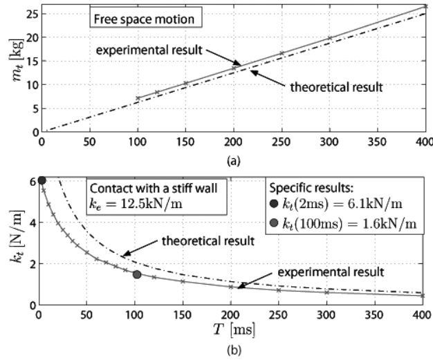
Fig. 8. Experimentally obtained displayed inertia m_t (a) and stiffness k_t (b) depending on round-trip delay T compared to theoretical results.
