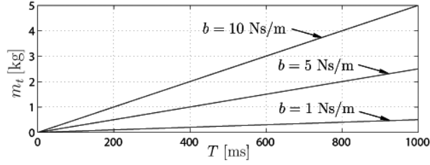
Fig. 4. Displayed inertia m_t in free space motion depending on round-trip time delay T and wave impedance b .
