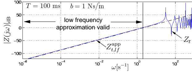
Fig. 2. Amplitude/frequency characteristics of the exact and the approximated displayed impedance in free space motion .
