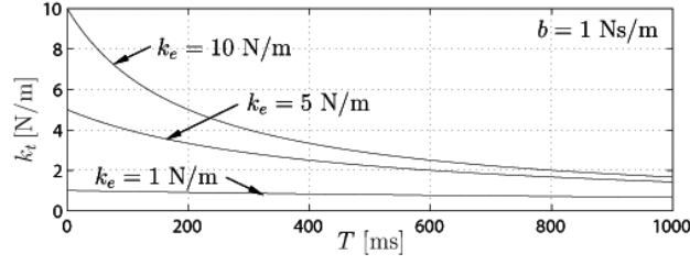
Fig. 5. Displayed stiffness k_t in contact with a stiff wall depending on round-trip time delay T and environment stiffness k_e .
