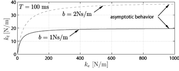
Fig. 6. Displayed stiffness k_t depending on environment stiffness k_e and wave impedance b .
