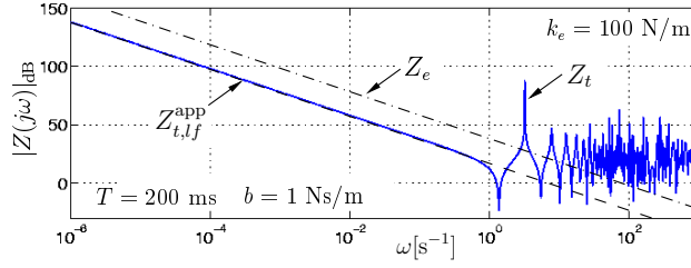
Fig. 3. Amplitude/frequency characteristics of the exact and the approximated displayed impedance in contact with a stiff wall .
