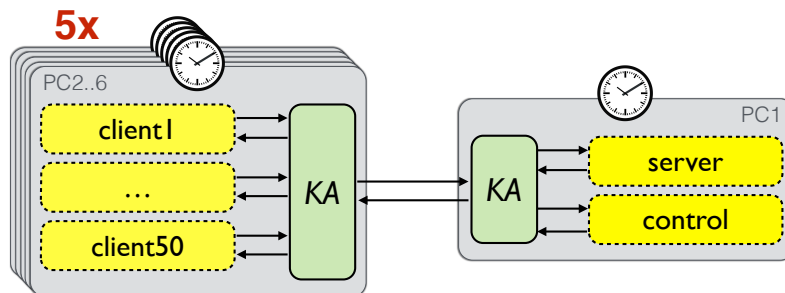
Figure 9.15: Small setup for the Latency-Between-Services measurement.
