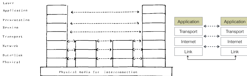
Figure 3.3: Left: the OSI architecture (original figure from [Zim80]); right: the TCP/ IP stack.
