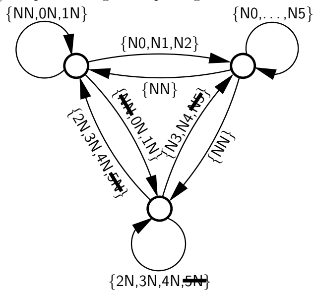
(c) Deletion of edges such that 8 outgoing edges per state remain.
