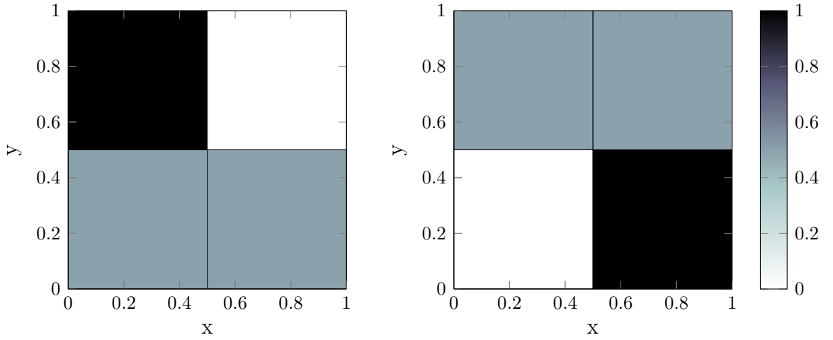
Figure 6.2.: Color map of \rho(\mathbf{P}_{1|0}) and \rho(\mathbf{P}_{1|1}) .
