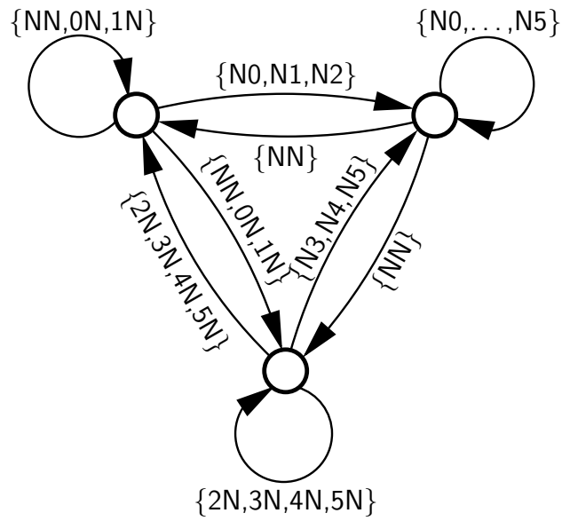
(b) Graph resulting from splitting the left state of G^2 .
