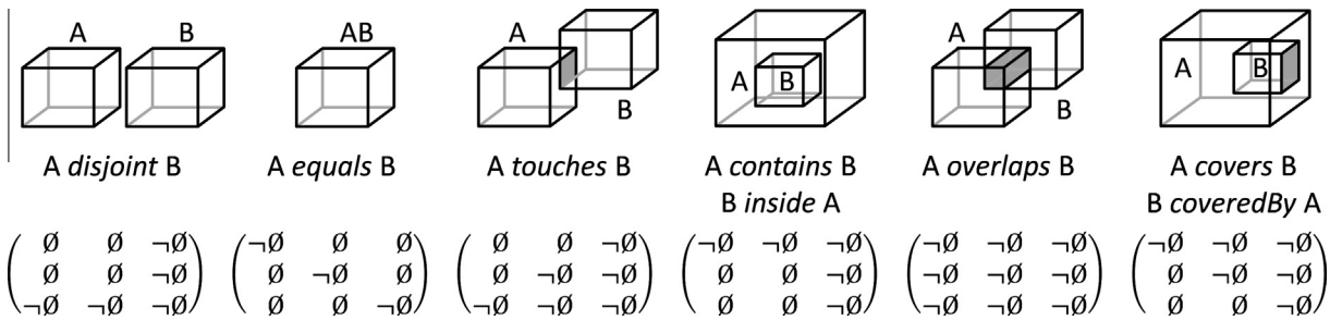
Fig. 2. The eight predicates defining the possible topological relationships between two solids in 3D.
