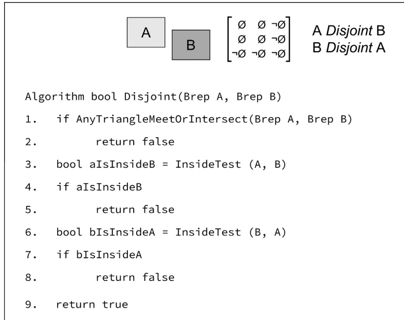
Fig. 6. Algorithm Disjoint.
