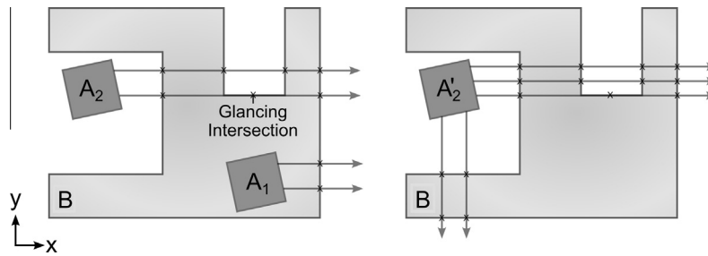
Fig. 5. Principle of the inside/outside classification of geometry objects based on ray tests.
