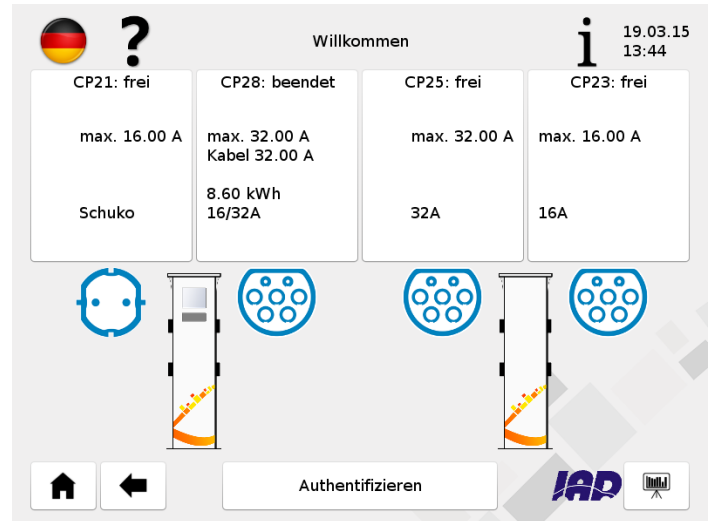
Fig. 4. Screenshot of the user interface (E-City-Routing charging station) as seen on the local touchscreen or in remote administration
