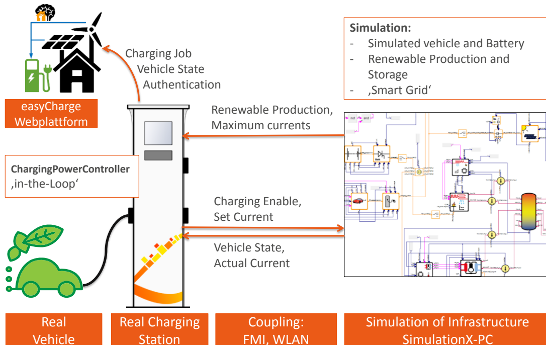
Fig. 7. FMI-connector overview: software under test and simulation model [2]
