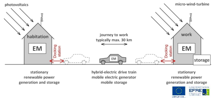
Fig. 2. Residence and Mobility - basic research to supply energy demands of home and commuting with local renewable energy [1]
