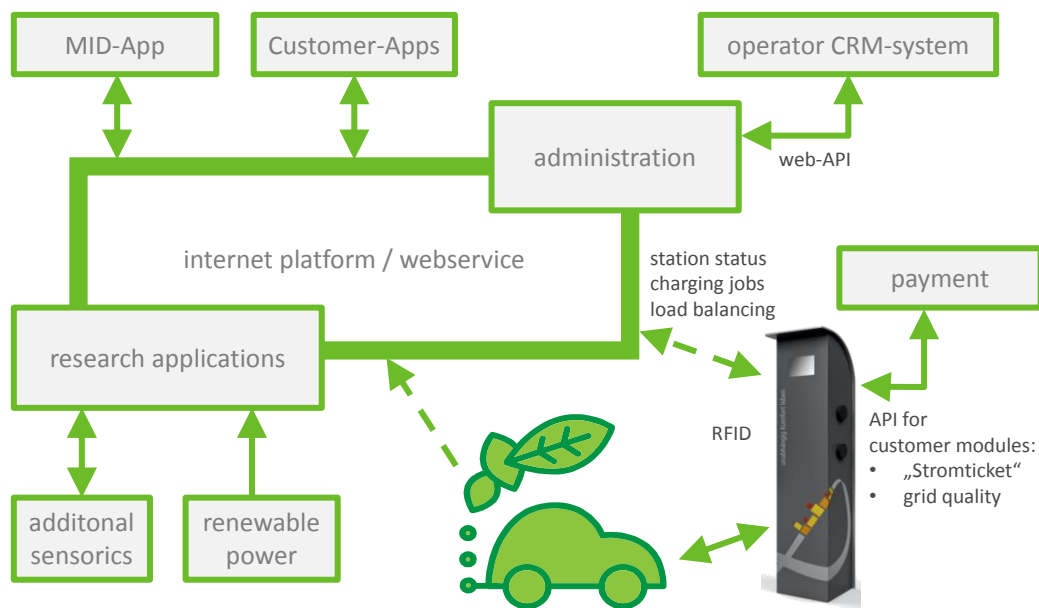
Fig. 3. easyCharge2 platform module
