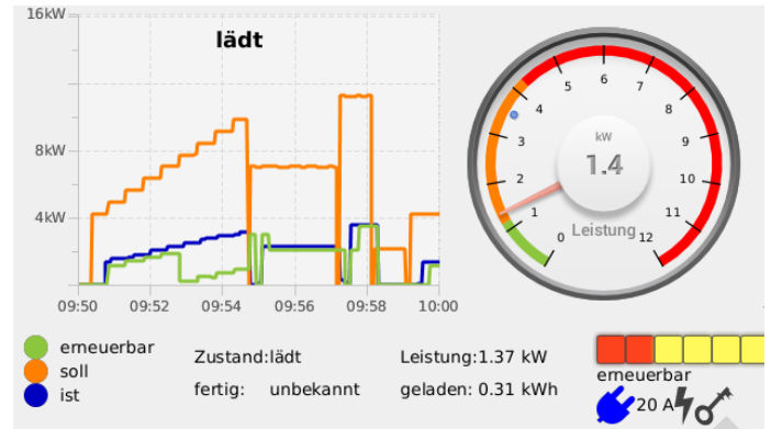
Fig. 6. Typical Test-Run of a on-phase Vehicle with the set current starting as a ramp and switching limits according to necessity
