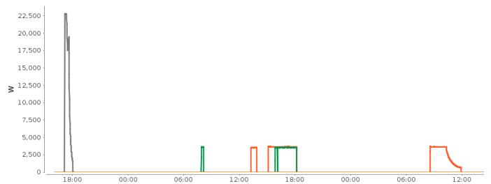
Fig. 1. Typical Load Profile for charging station with 4 Outlets (2x 32A, 2x 16A)
