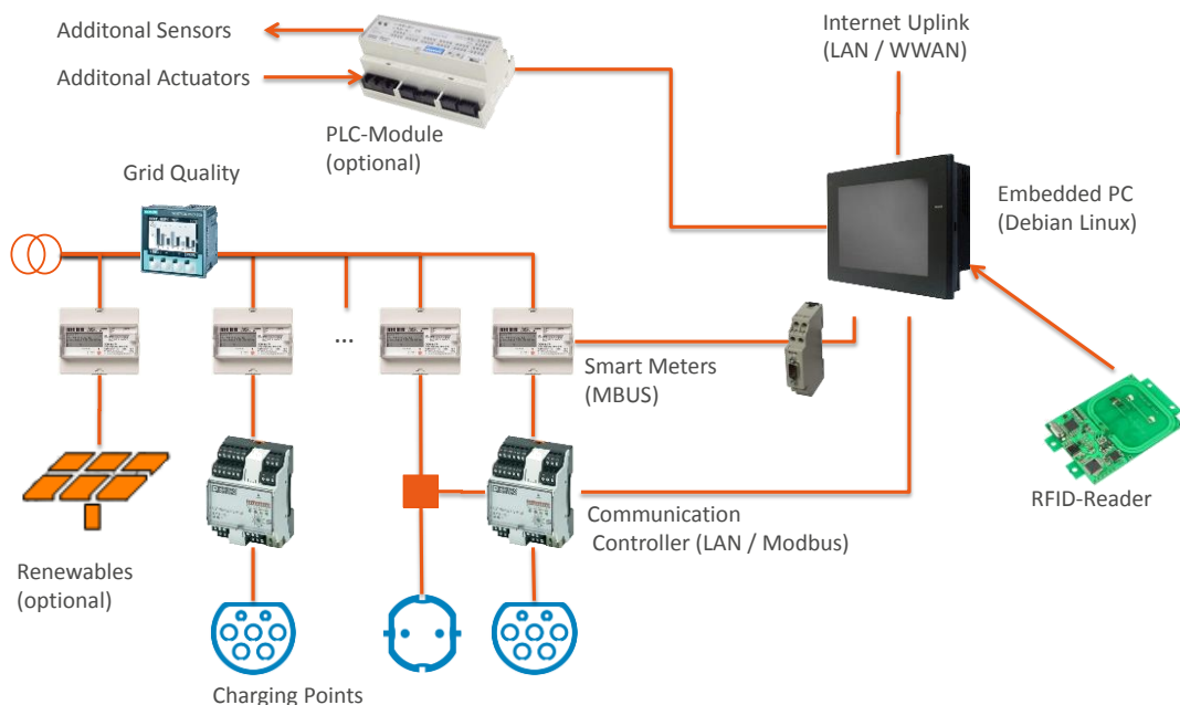
Fig. 5. System layout for a master-slave charging concept with a central control unit and several wallboxes [3]
