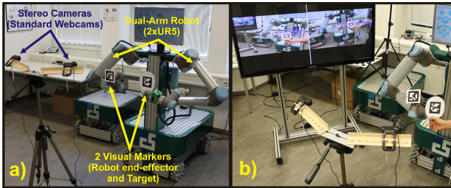
Fig. 5. This figure shows in a) the experimental setup used to validate our approach. It is composed of a dual-arm mobile manipulator, where 2 UR-5 robots are used as arms. The right arm is equipped with a AR marker mounted on its end-effector. The stereo-camera setup comprises two standard webcams logitech pro9000 mounted on a tripod. The system has been calibrated with respect to the body of the robot. In b) is depicted a snapshot of the task, where the target marker is moved by the user. The goal is to visually track the pose of the target marker with the robot arm.
