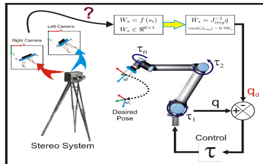
Fig. 1. A classical problem of visual servoing is to generate a full-rank mapping between the visual feature space s \in \mathbb{R}^{2m \times 1} and the joint velocity space \dot{q} \in \mathbb{R}^{n \times 1} to design dynamic controls for robots \tau \in \mathbb{R}^{n \times 1} [Nm] .
