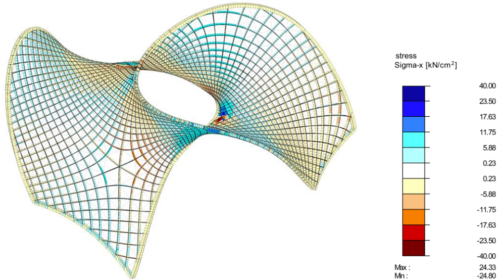
Figure 12: Surface stresses of the grid structure resulting from both the elastic erection process and self-weight.
