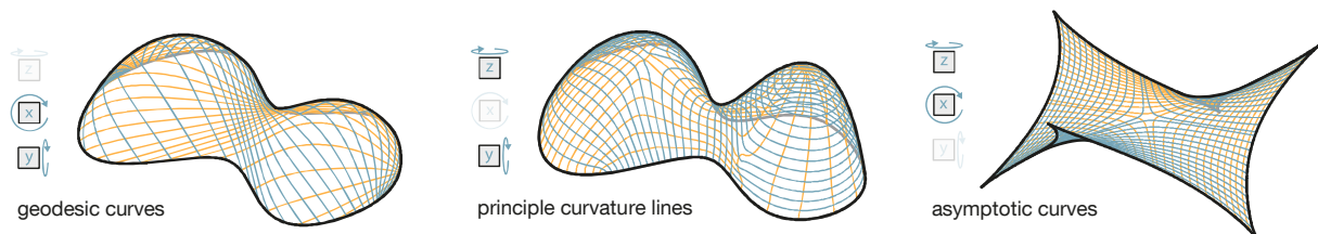
Figure 4: Surface-curves have three curvatures: Geodesic curvature (z), geodesic torsion (x), and normal curvature (y). For each of them, if avoided, a related curve type exists: geodesic curves, principle curvature lines and asymptotic curves.
