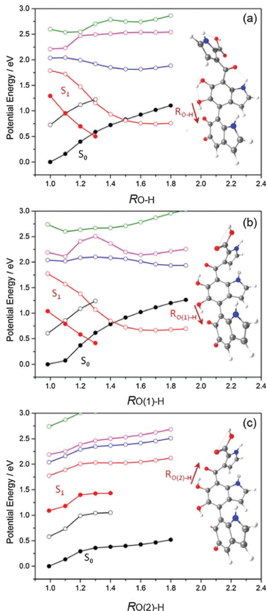
Fig. 6 Potential energy profiles of the S_0 (black), S_1 (red), S_2 (blue), S_3 (pink) and S_4 (green) states along the R_{O-H} coordinate – representing intramolecular proton transfer in structures E (a) and F ((b) & (c)).
