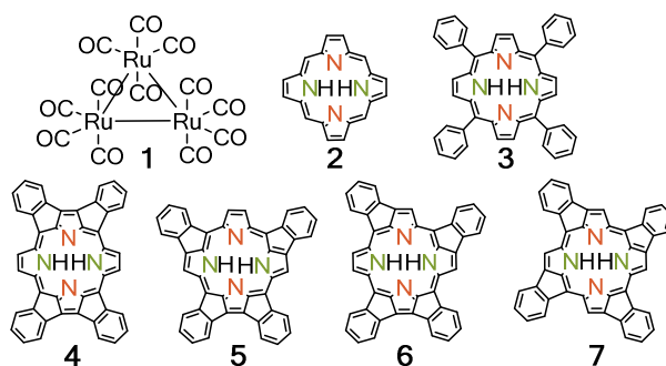
Figure 1. Molecular structures of the Ru 3 (CO) 12 metal precursor 1 , porphine (2H-P) 2 , meso -tetraphenylporphyrin (2H-TPP) 3 , and the planar 2H-TPP derivatives 4 , 5 , 6 , 7 . Green and orange indicate the aminic and iminic N sites of the porphyrin macrocycle, respectively.
