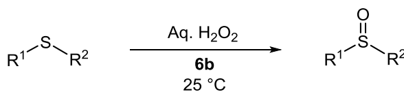
Scheme 2. Oxidation of sulfides to sulfoxides mediated by WCCWCA 6b .
