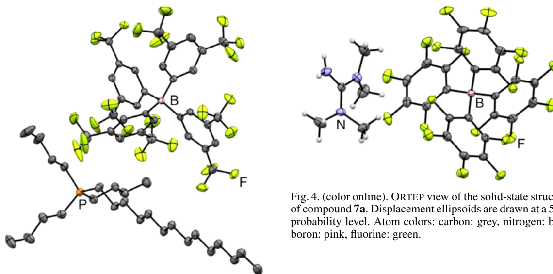
Fig. 3. (color online). ORTEP view of the solid-state structure of compound 6b . Displacement ellipsoids are drawn at a 50% probability level. Hydrogen atoms are omitted for clarity. Atom colors: carbon: grey, phosphorus: orange, boron: pink, fluorine: green.
