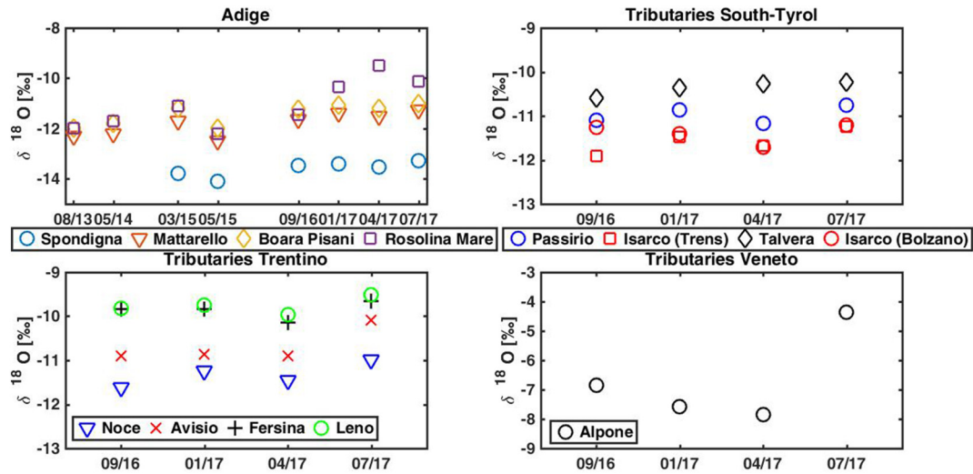
Fig. 3. Temporal variability of \delta^{18}\text{O} in four gauging stations along the Adige river and some of its tributaries. Data for the Adige in 2013, 2014 and 2015 are from Natali et al. (2016).
