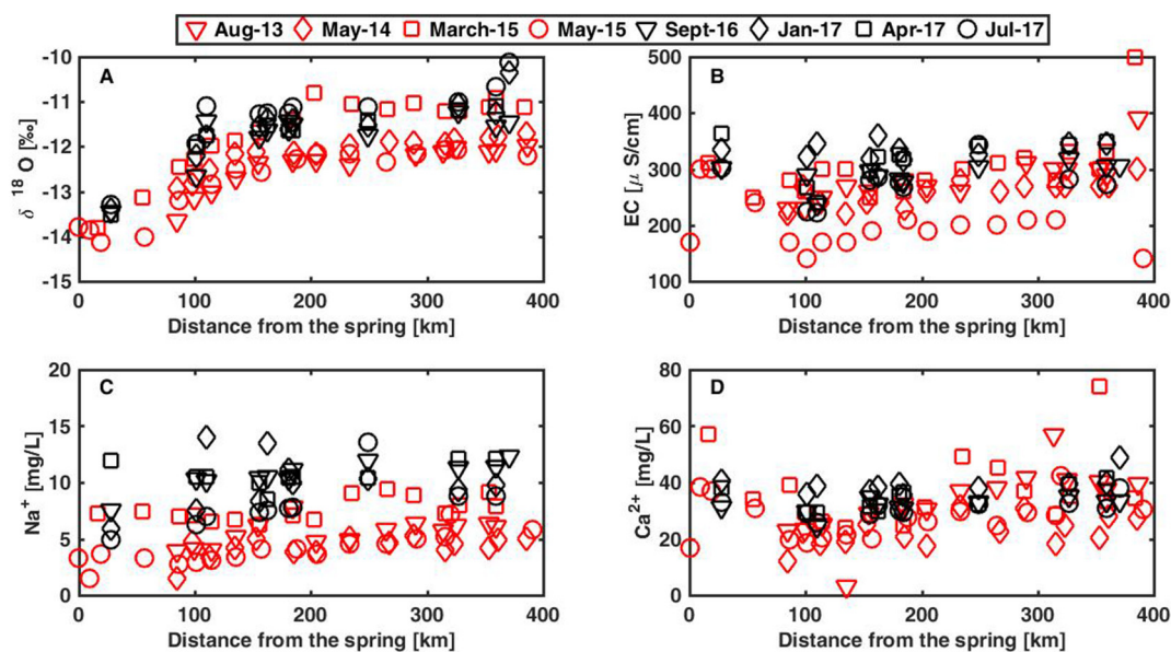
Fig. 6. Variability of δ 18 O (panel A), EC (panel B), Na + (panel C) and Ca 2+ (panel D) along the Adige River. Notice that the values of EC, Na + and Ca 2+ for the last sampling point (after barrier) collected in 2017 are not shown since they are out of range (see Tables 2 to 5). Data for the Adige in 2013, 2014 and 2015 are from Natali et al. (2016).
