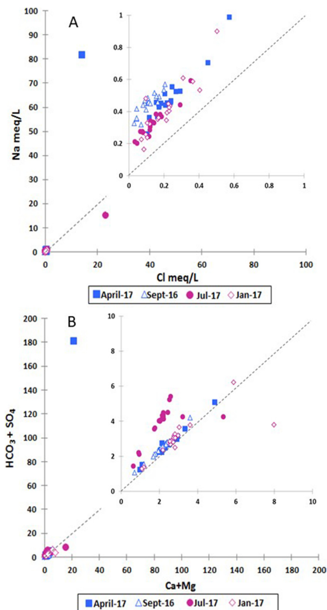
Fig. 8. Ionic ratios: (A) Na versus Cl; (B) Ca + Mg versus HCO 3 + SO 4 .
