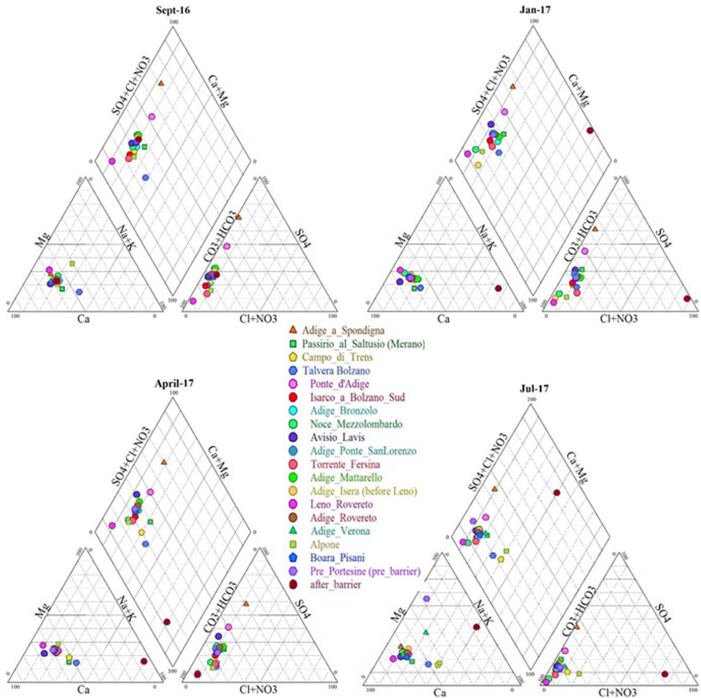
Fig. 7. Piper diagram diagrams for the Adige catchment and its tributaries.
