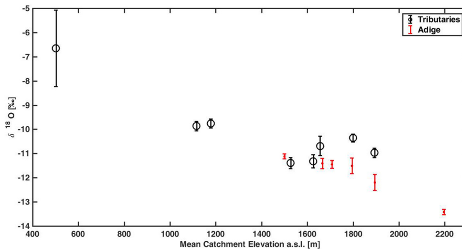
Fig. 4. Variability of \delta^{18}\text{O} as a function of the mean catchment elevation of the subbasins (Passirio, Talvera, Isarco, Avisio, Noce, Leno, Fersina and Alpone, in decreasing order of mean catchment elevation) and the Adige catchment closed at six different gauging stations (Spondigna, Ponte d'Adige, Bronzolo, Mattarello and Boara Pisani, in decreasing order of mean catchment elevation), with circles and dots respectively.
