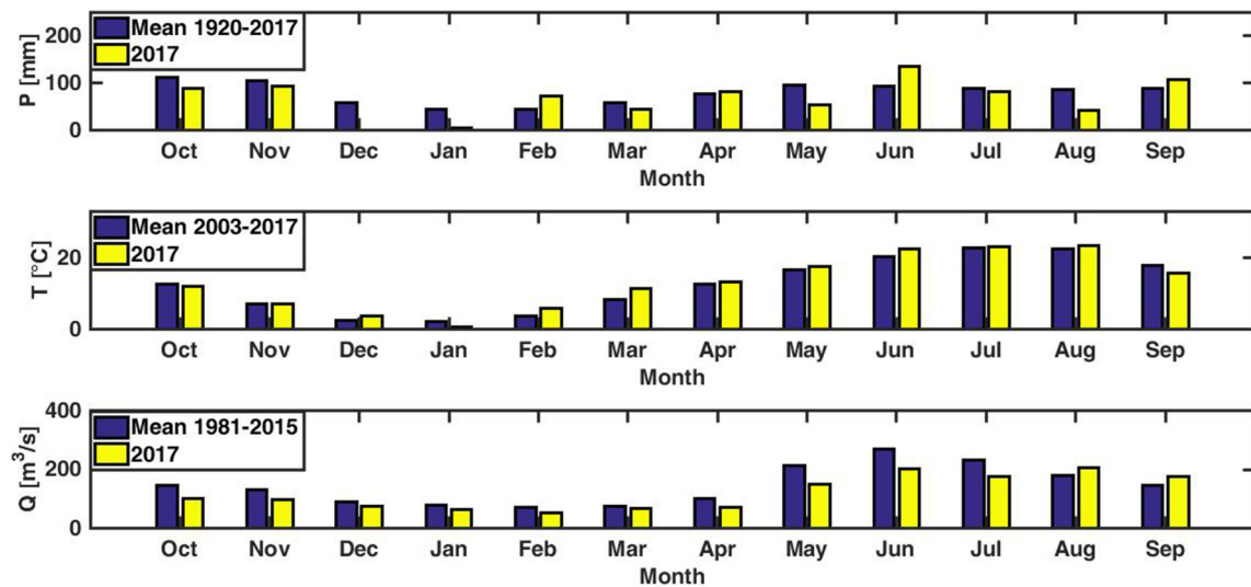
Fig. 2. Comparison between cumulative monthly precipitation of the hydrological year 2017 and the mean from 1920 to 2017 for the station Trento Laste (upper panel); Comparison between mean monthly temperature of the hydrological year 2017 and the mean from 2003 to 2017 for the station Trento Laste (central panel); comparison between mean monthly discharge of the hydrological year 2017 and the mean monthly discharge computed over the period 1981–2015 for the gauging station Bronzolo (lower panel).
