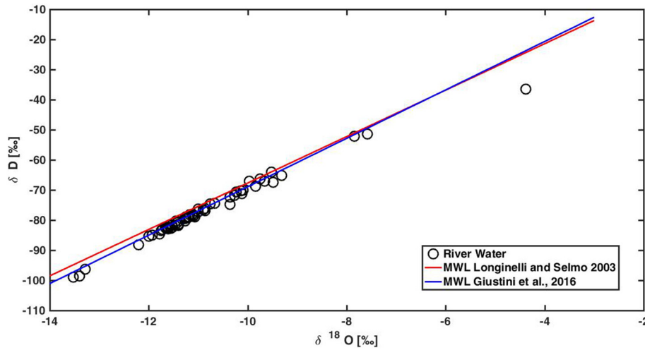
Fig. 5. Comparison between the of \delta D - \delta^{18}O isotopic signature of the river water samples collected in this study and the local meteoric water line proposed by Giustini et al. (2016), i.e., \delta D = 8.04 \cdot \delta^{18}O + 11.47 and Longinelli and Selmo (2003), i.e., \delta D = 7.7094 \cdot \delta^{18}O + 9.4034 .
