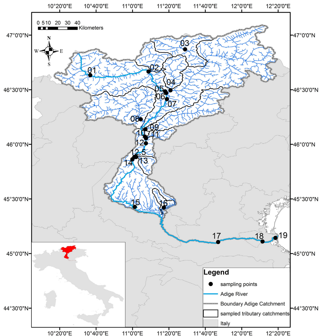
Fig. 1. The Adige catchment and the sampling locations (the name of the sampling points are reported in Table 1). The boundary of the sampled tributary catchments is indicated with a black contour line.
