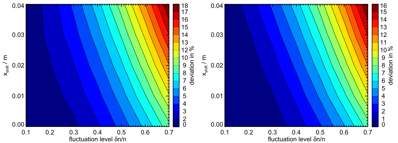
Figure 10. Polynomial fit to the deviation of beam broadening obtained from fitting (left) a Gaussian ( \chi^2 \approx 2.3 using all 35 beam broadening values) and (right) a Cauchy distribution ( \chi^2 \approx 1.6 using all 35 beam broadening values) to detector antenna signals at x = 2.31 m for WKBeam calculations with respect to full-wave simulations (i.e. overestimation of WKBeam calculations compared to the full-wave simulations).
