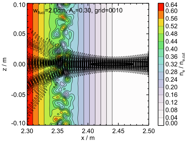
Figure 7. Same as figure 4, but with the turbulence layer shifted to the left ( A_0 = 0.30 , w_{\text{fluct}} = 2 cm, x_{\text{shift}} = 4 cm, see equation (14)).
