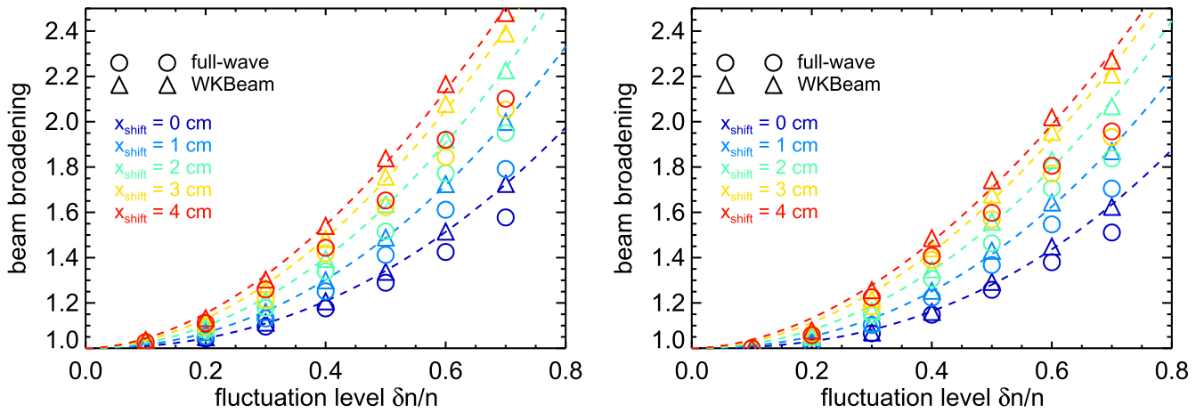
Figure 9. Beam broadening as a function of the fluctuation amplitude at a detector antenna position of x = 2.31 m from full-wave simulations and WKBeam calculations as deduced from (left) Gaussians and (right) from Cauchy distributions fitted to the detector antenna signals. Power laws are fitted to the WKBeam results (dashed lines).
