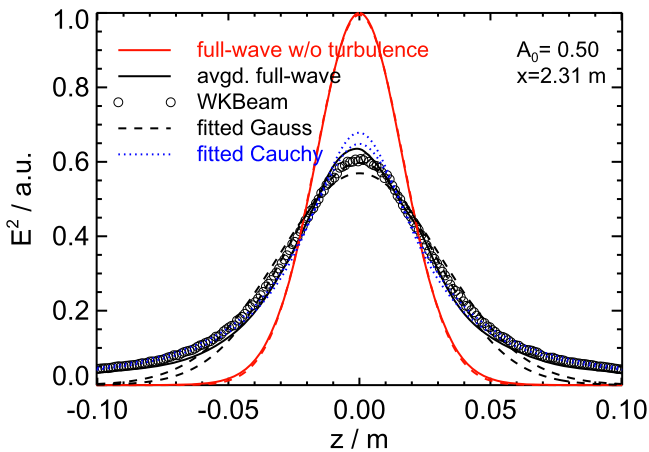
Figure 8. Detector antenna signals at a radial position of x = 2.31 m from full-wave simulations and WKBBeam calculations with Gaussians and Cauchy distributions fitted to them for A_0 = 0.50 and x_{\text{shift}} = 4 cm.
