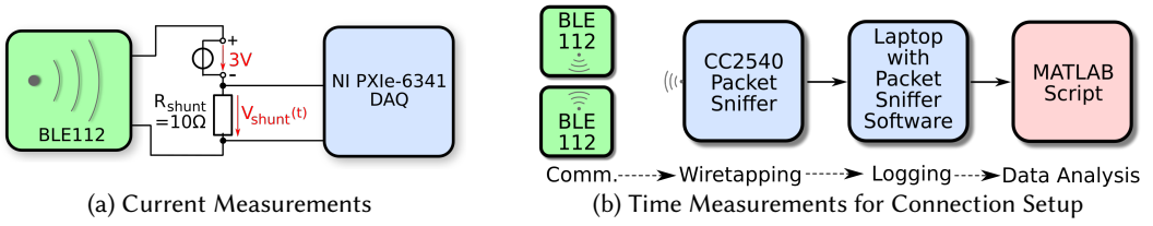
Fig. 6. Measurement Setups
