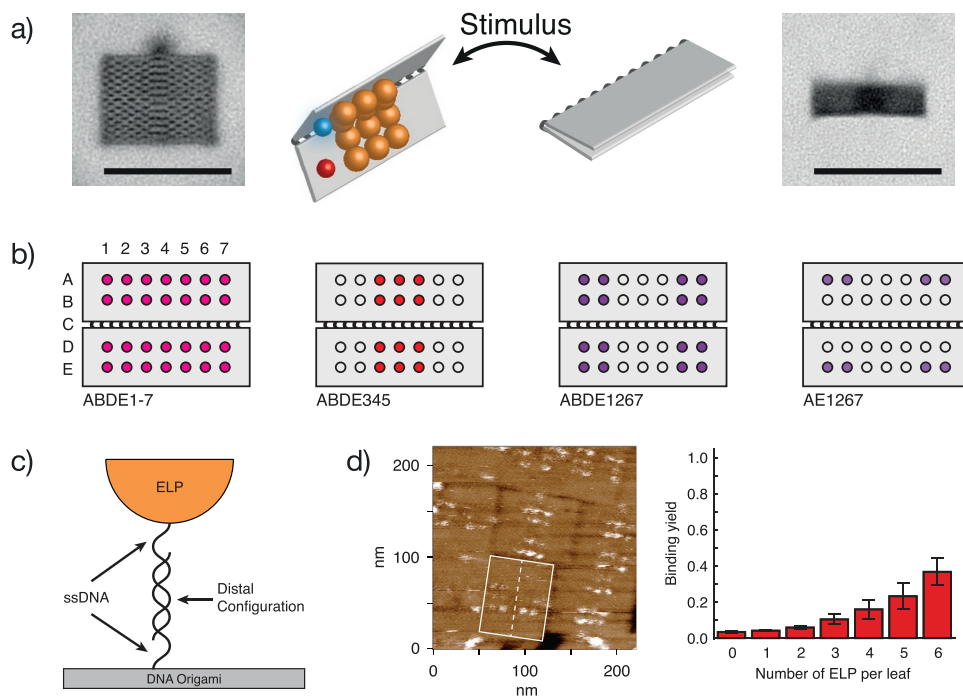
Figure 1. DNA origami design and ELP configuration. a) Class-averaged TEM images of an open rectangle (left) and a closed rectangle (right). Center: Illustration of the working principle and the rectangle design with ELPs (orange spheres) and dyes (red and blue). Scale Bar: 100 nm. b) Graphical representation of four exemplary ELP-rectangle configurations. c) Illustration of the binding site design in distal configuration. d) Left: Representative AFM image of the rectangle with attached ELPs in ABDE345 configuration. Right: Binomial distribution of the ELP-occupied binding sites per leaf. The given uncertainties are standard deviations.
