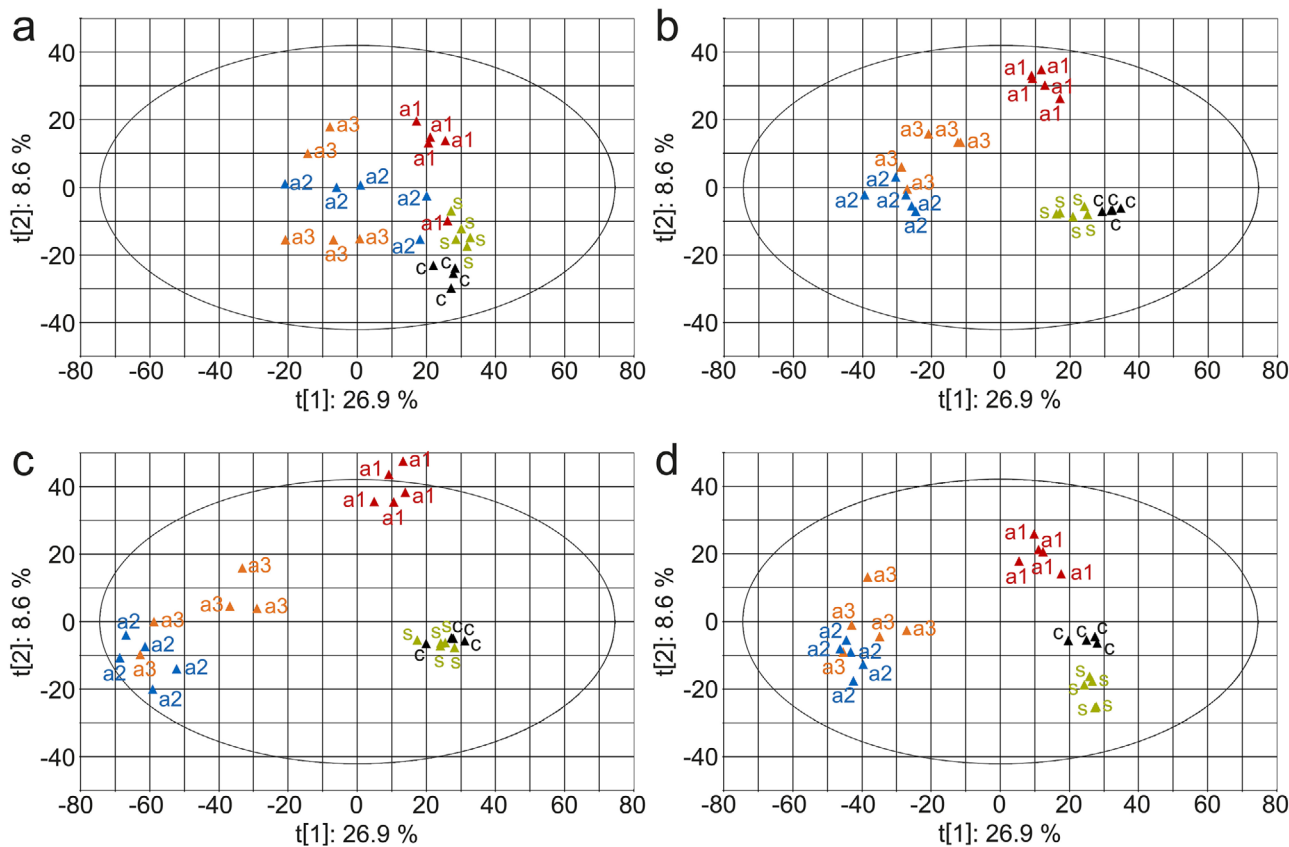
Figure 7. Scatter plots of the principal component analysis (PCA) of the FTICR-MS data. The plots display A. solani (▲,s), the three A. alternata isolates 1 (▲,a1), 2 (▲,a2), and 3 (▲,a3) and the control samples (▲,c) on the 4th day (a), the 7th day (b), the 9th day (c), and the 11th day (d) of cultivation.
