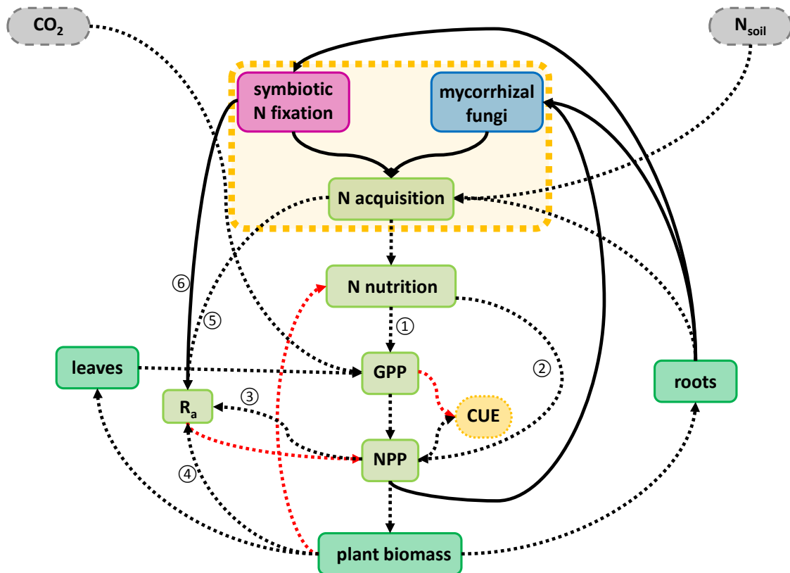
Figure 5.1.: Schematic representation of implications of the implementation of symbiotic N fixation (pink box) and mycorrhizal fungi (blue box) into a TBM on simulated plant growth.
