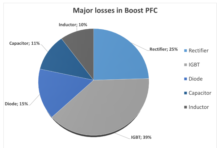
Figure 21 Average power losses in a boost PFC with Full-Si IGBT obtained from simulation at R_g = 12 \Omega , V_{dc} = 400 V , P_o = 3.3kW and f_{sw} = 80kHz
