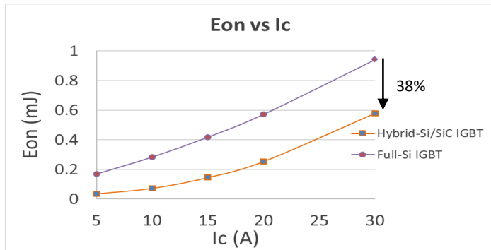
Figure 19 Turn on energy as a function of device current for Full-Si IGBT and Hybrid-Si/SiC IGBT at R_g = 5 \Omega , V_{dc} = 400 V , T_j = 25^\circ C
