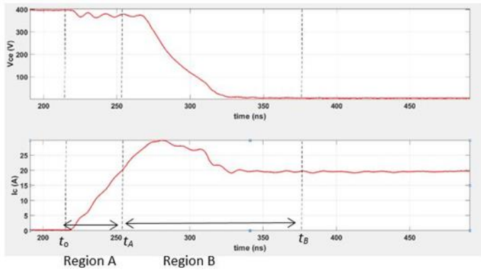
Figure 3 Split-up of the turn on event
