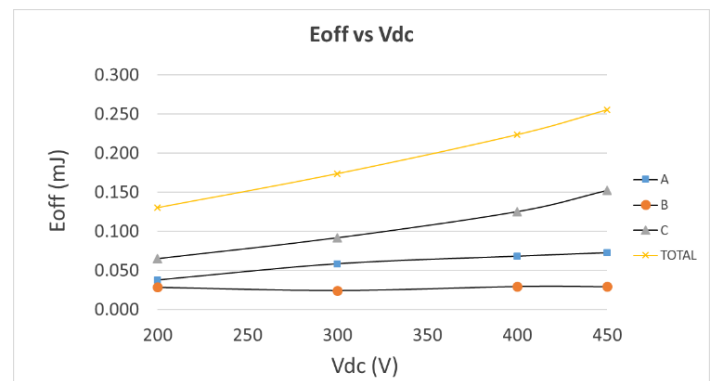
Figure 17 Turn off energy arising from its different root causes as a function DC link voltage (Full-Si IGBT) at V_{dc} = 400 V, R_g = 14.6 \Omega and I_c = 20 A A = capacitive, B = commutation, C = tail current
