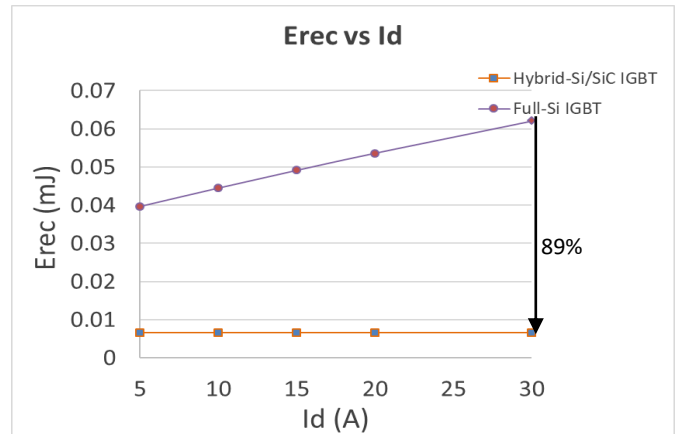
Figure 20 Reverse recovery energy as a function of device current for Full-Si IGBT and Hybrid-Si/SiC IGBT at R_g = 5 \Omega , V_{dc} = 400 V , T_j = 25^\circ C
