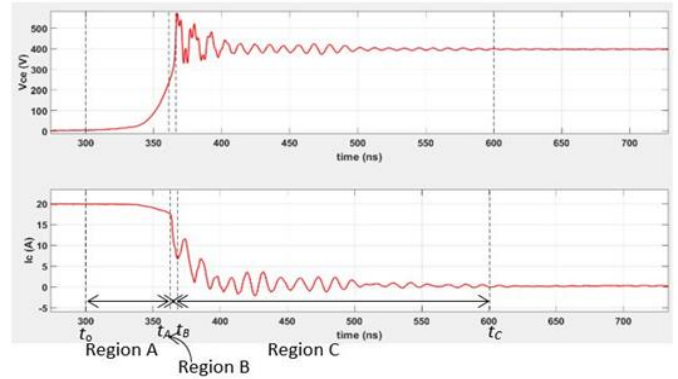
Figure 4 Split-up of the turn off event
