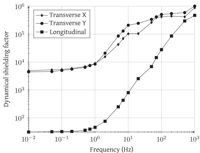
FIG. 4. Measurement of the dynamical shielding factor at the center of the shield with end-caps installed. Effective eddy current shielding the aluminum pipe used as a guide for the probe is visible through the increased shielding factor at frequencies above 1 Hz.
