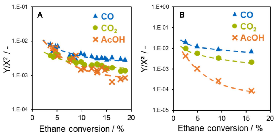
Fig. 7 Second rank delplots for ethane oxidation over Q-M1 (a) and B-M1 (b) samples. Reactions conditions applied: T = 290\text{--}370\text{ }^{\circ}\text{C} (Q-M1), 330\text{--}420\text{ }^{\circ}\text{C} (B-M1); \text{C}_2\text{H}_6:\text{O}_2:\text{inert} = 3\text{:}9\text{:}3\text{:}9\text{:}82\text{:}94 (Q-M1), \text{C}_2\text{H}_6:\text{O}_2:\text{inert} = 9\text{:}9\text{:}82 (B-M1); p = 1.5\text{--}4.0\text{ bar(a)} (Q-M1), 1.0\text{ bar(a)} (B-M1); \text{WHSV} = 4.8\text{--}19.0\text{ h}^{-1} (Q-M1), 4.8\text{ h}^{-1} (B-M1)
