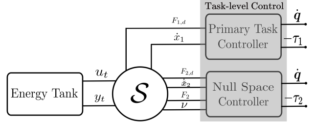
Fig. 2. Interconnection of the energy tank with the primary, null space tasks controllers. The gray block Task level Control corresponds to the same block in Fig. 1
