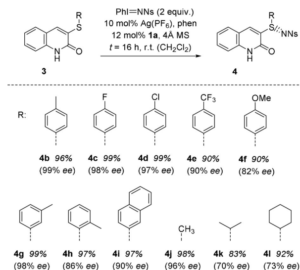
Scheme 5. Enantioselective Ag-catalyzed sulfimidation of various 3-thio-substituted 2-quinolones 3 employing ligand 1a as the source of chirality (60 μmol scale, substrate concentration c = 10 mM). The enantiomeric excess ( ee ) was calculated from the ratio of enantiomers ( 4/ent-4 ) as determined by chiral HPLC analysis.
