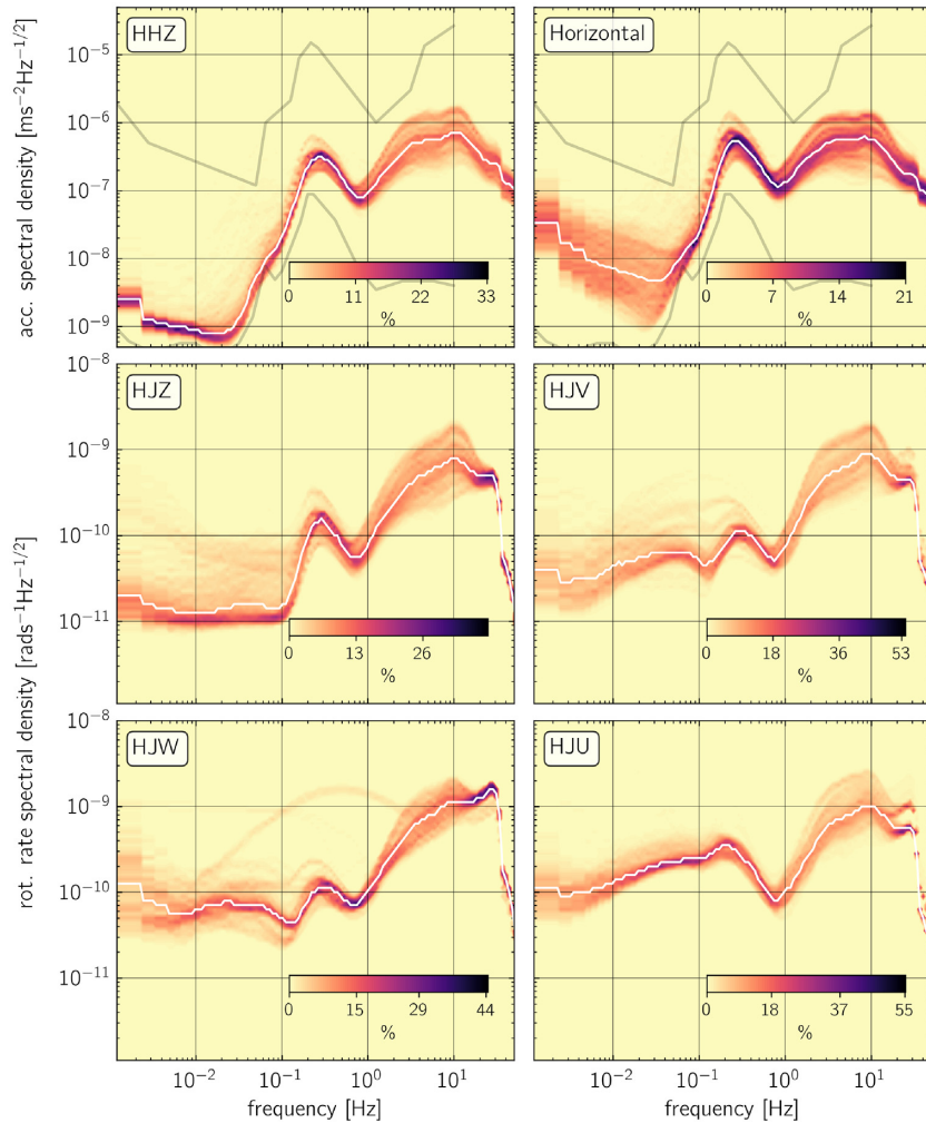
Figure 9. PPSDs for the co-located vertical and horizontal components of the broadband station FUR (top row) and all four ROMY components. The white line indicates the median of the distributions. 1 hr time windows with 50 per cent overlap were used to calculate power spectral densities. For ROMY PPSDs, we used around 30 continuous recordings each lasting 6 hr during periods of stable operation. In order to demonstrate station performance at low background noise levels, we exclude strong signals from nearby noise sources like farming machinery, with peak signal amplitudes exceeding 100 \text{ nrad s}^{-1} .
