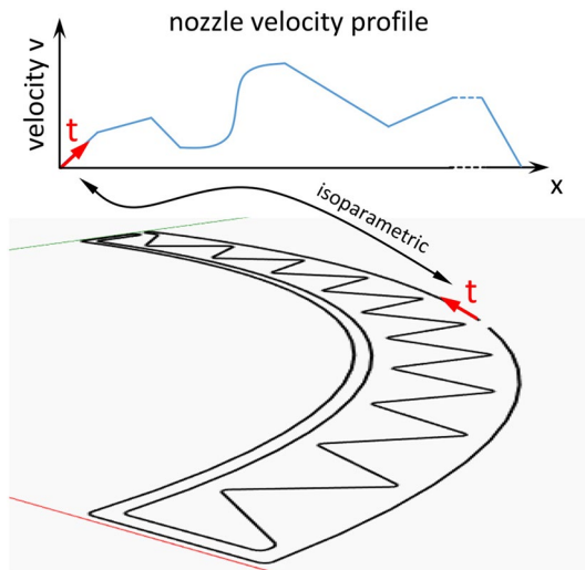
Fig. 12 Qualitative example of non-constant parameter modeling using an IfcCurve that is “isoparametric” to the print path
