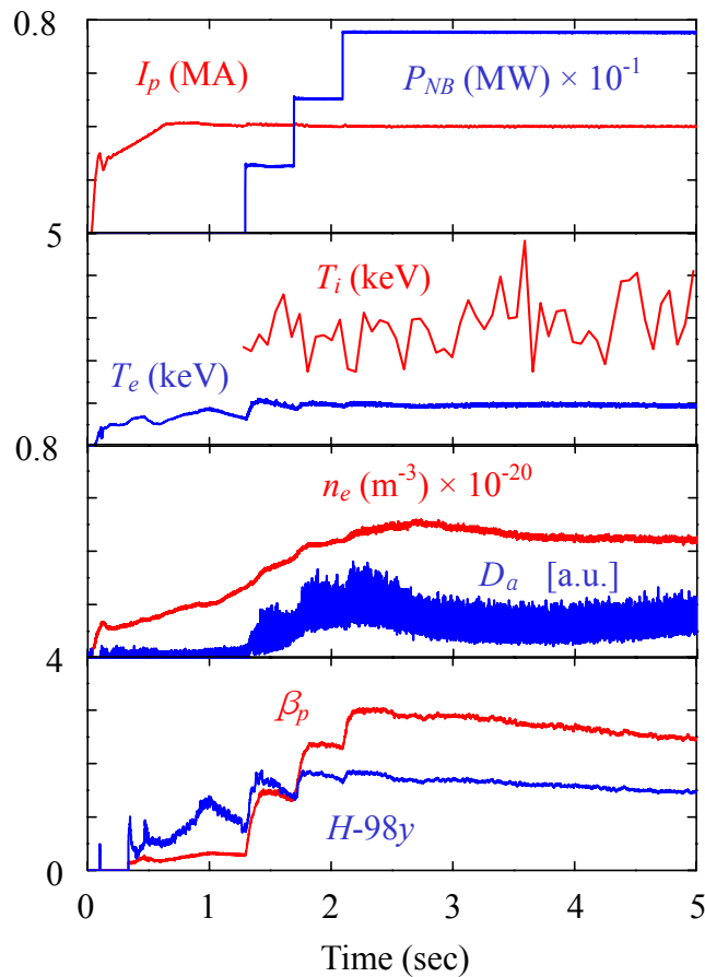
Figure 3.1. Time traces of plasma current, NB heating power (beam sources 3, 7, 6 are used), central ion temperature and averaged electron temperature, line-averaged electron density, D_\alpha , poloidal beta, H_{98}(y,2) of pulse 13686 in ASDEX Upgrade.
