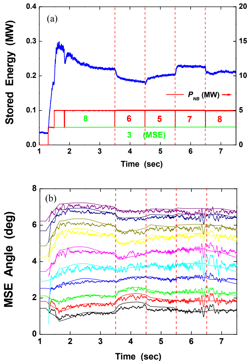
Figure 4.9. Pulse 17530 at ASDEX Upgrade; stored energy and beam power is presented in (a), beam source is changed at 3.5sec to source 6, at 4.5sec to source 5, at 5.5sec to source 7 and at 6.5sec to source 8. Time points where the beam source is changed are presented in vertical dashed lines. MSE angles from the experiment (with small oscillations) and the ASTRA simulation are presented in (b).
