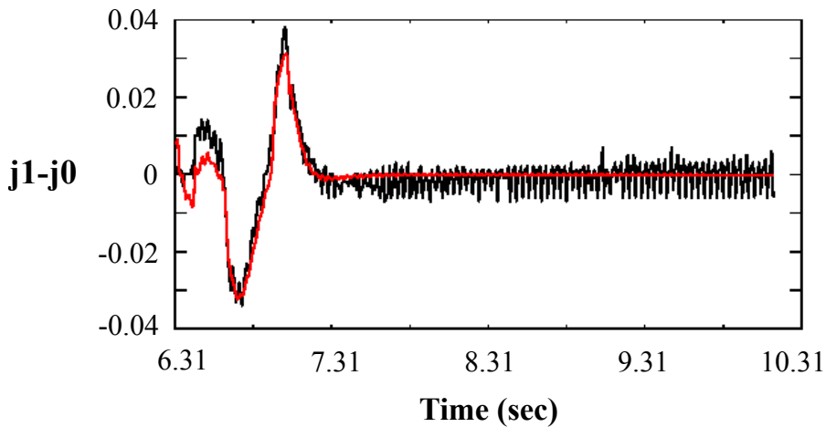
Figure 4.3. Time variation of current density ( j_1-j_0 ) at r = 0.225\text{m} for the step response of beam source 8 ( \Delta P_{NB} ). The dark line (in black) represents reference signal ( y ); computed by ASTRA code and the light line (in red) represents predicted output signal ( y_{sim} ); computed by the 15 th state-space model.
