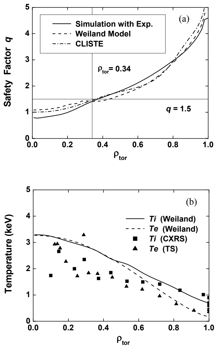
Figure 2.6. q -profiles (a) and temperature profiles (b) in the high \beta_N discharge with NTM's (pulse 14517) at 3.6sec.
