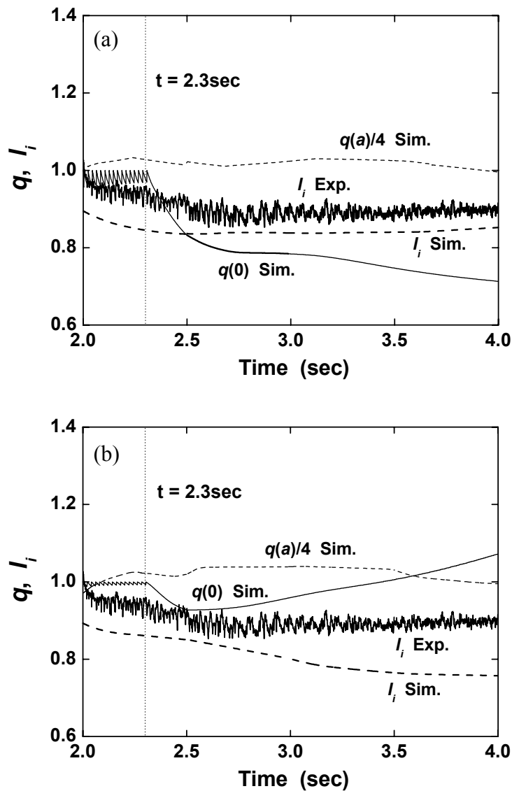
Figure 2.3. The time evolution of internal inductance ( I_i ), q -values at the centre ( q_0 ) and at the edge ( q_a ) in the simulation using experimental temperature profiles (a) and using the Weiland model (b) for the high \beta_N discharge (pulse 14521).
