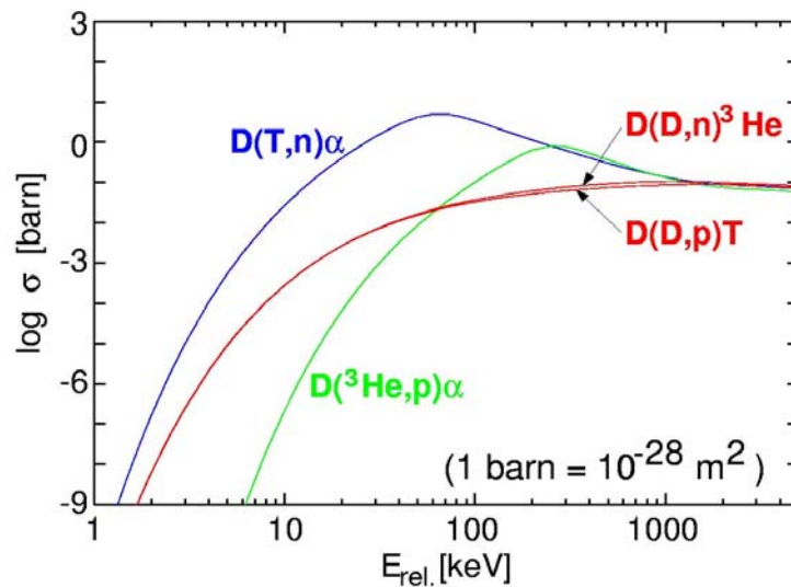
Figure 1.1. Cross section for the reactions D-T, D-D and D- 3 He. The two D-D reactions have similar cross sections.
