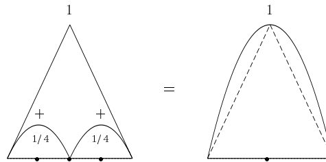
Figure 6: Switching from fine to coarse level with quadratic hierarchical basis functions.
