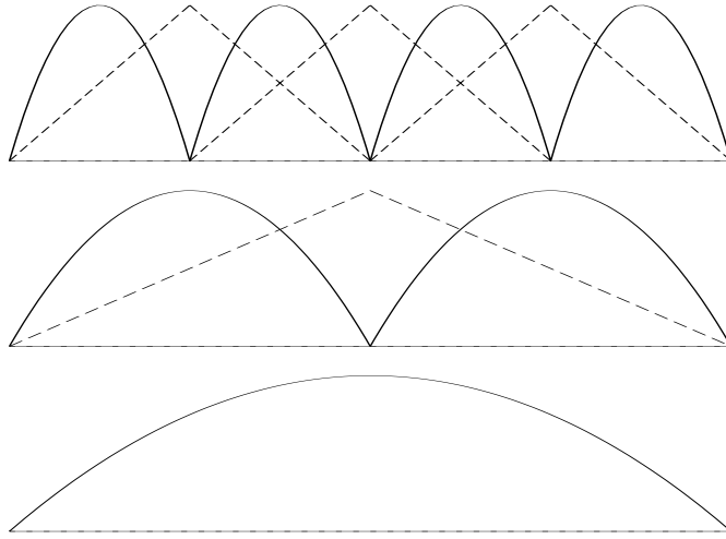
Figure 7: Quadratic hierarchical basis and nodal point bases on each level.
