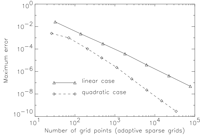
Figure 12: Maximum error vs. number of grid points (linear and quadratic case).
