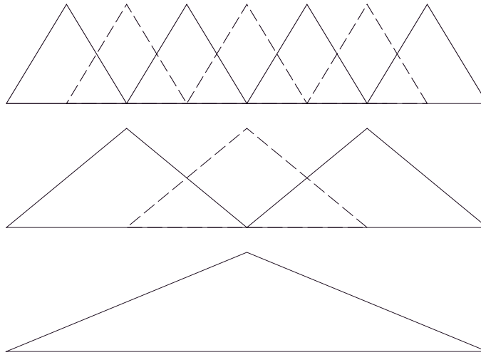
Figure 5: Linear hierarchical basis and nodal point bases on each level.
