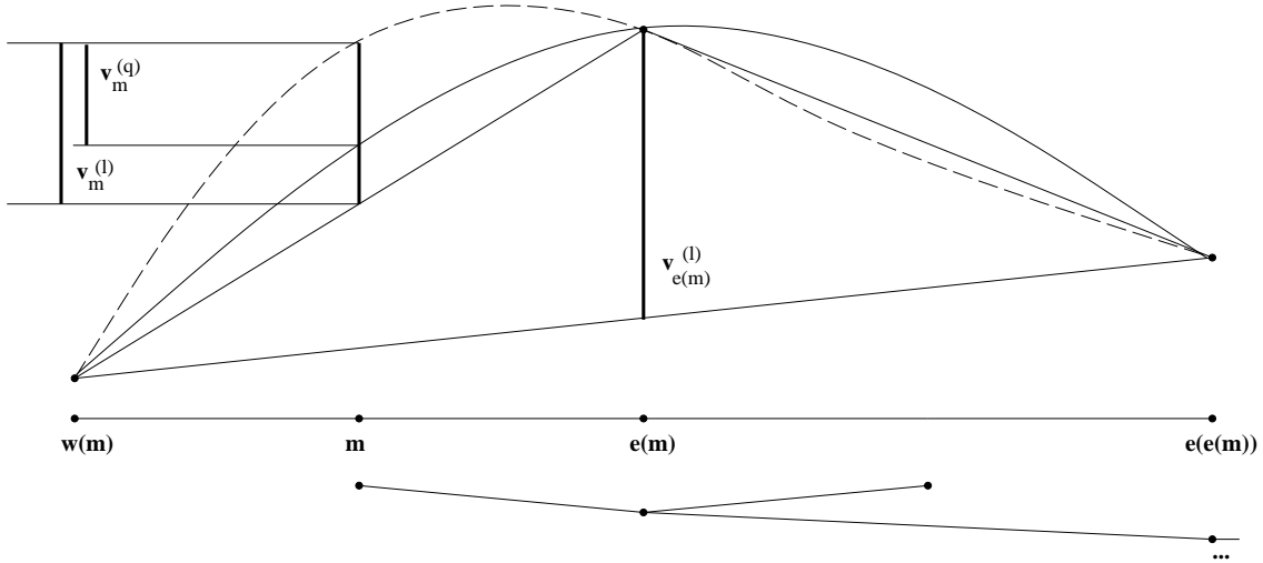
Figure 8: Linear and quadratic hierarchical surplus.
