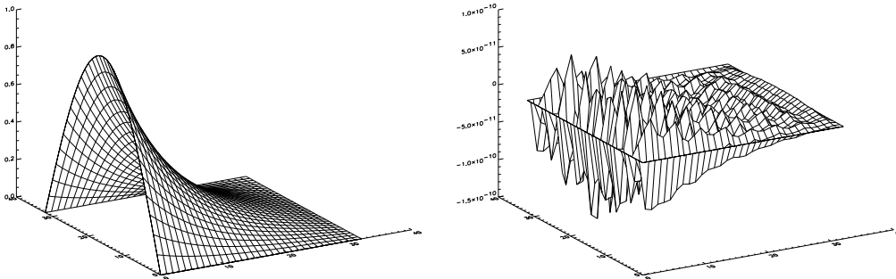
Figure 10: Sparse grid solution (left) and error (right) of the model problem.
