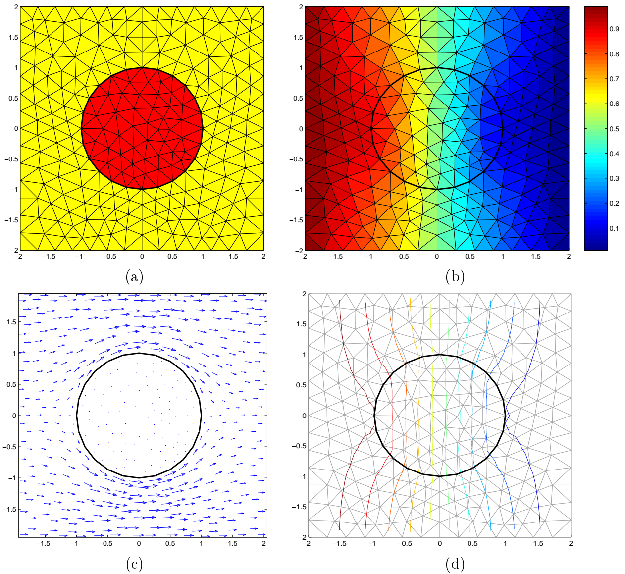
Figure 7: Circle problem: (a) grid with material properties, (b) temperature distribution, (c) heat flux distribution, (d) temperature contour isolines
