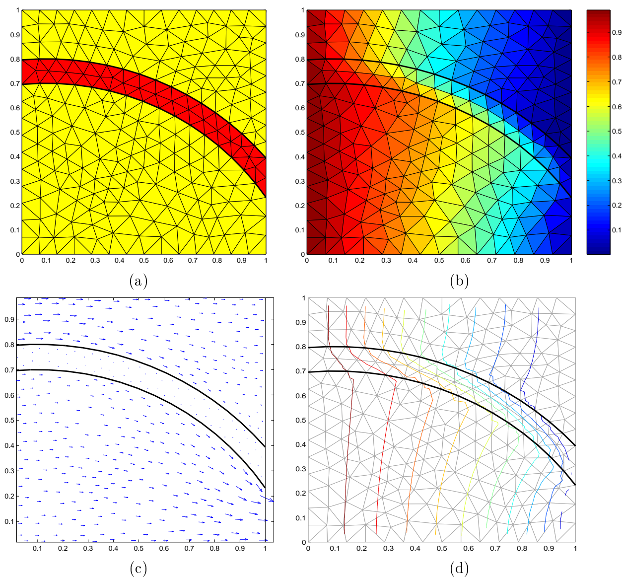
Figure 9: Streak problem: (a) grid with material properties, (b) temperature distribution, (c) heat flux distribution, (d) temperature contour isolines
