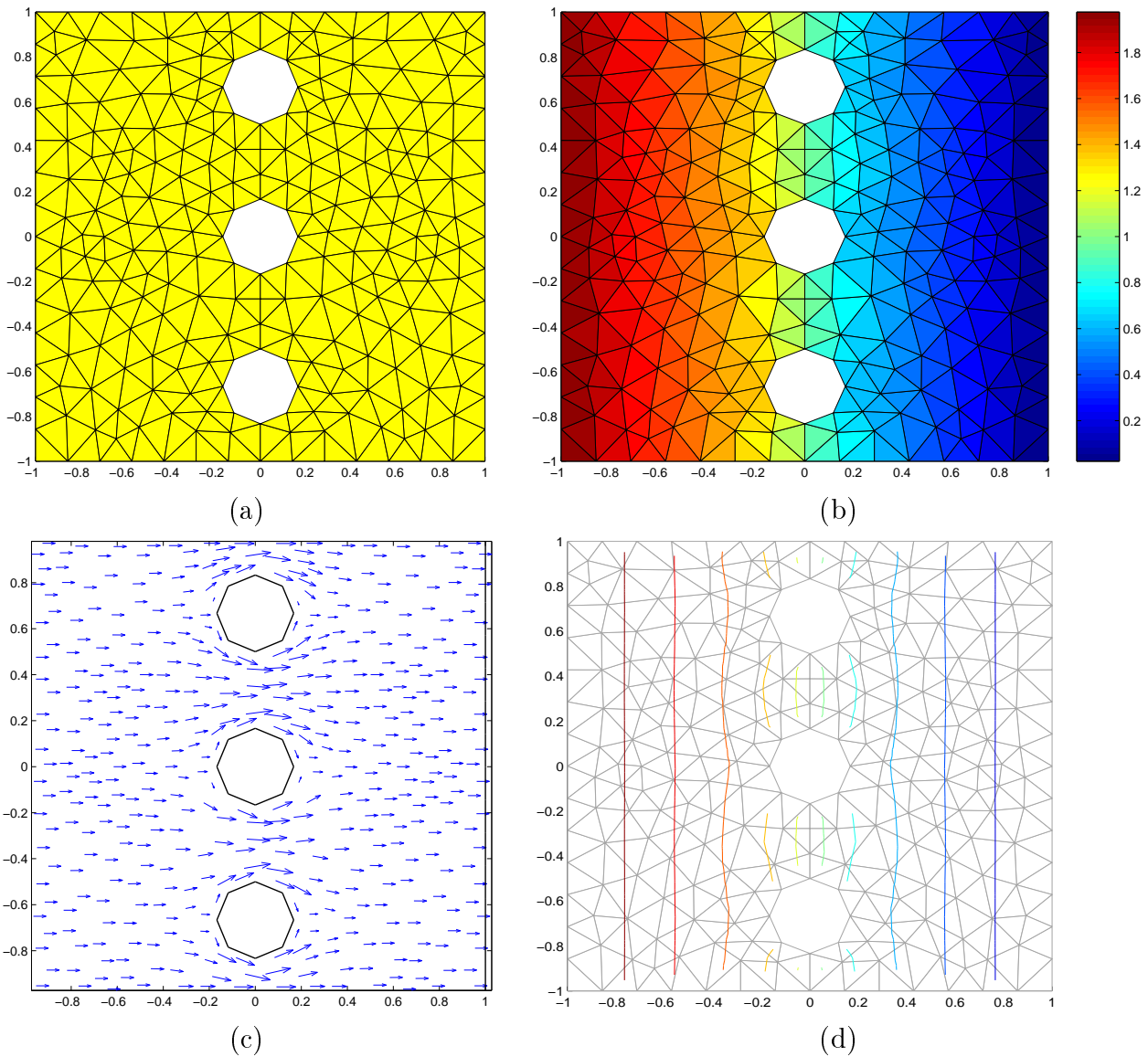
Figure 10: Three holes arranged vertically problem: (a) grid with material properties, (b) temperature distribution, (c) heat flux distribution, (d) temperature contour isolines
