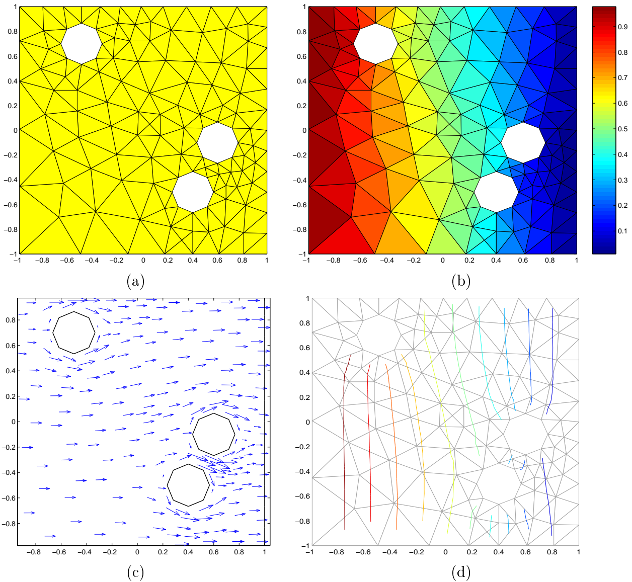
Figure 11: Three holes arranged randomly problem: (a) grid with material properties, (b) temperature distribution, (c) heat flux distribution, (d) temperature contour isolines
