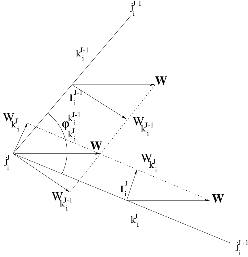
Figure 4: Projections of the vector \mathbf{W} on two edge normals is moved into the join vertex of these two edges for computing the inner product (\mathbf{A}, \mathbf{B})_{j_i^J} in triangle i with respect to the vertex j_i^J .
