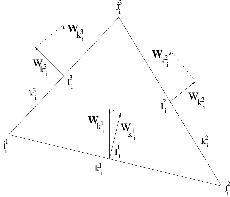
Figure 3: Vector function \mathbf{w} is represented by the projection of the vector on the edge normals at centers of the edges.
