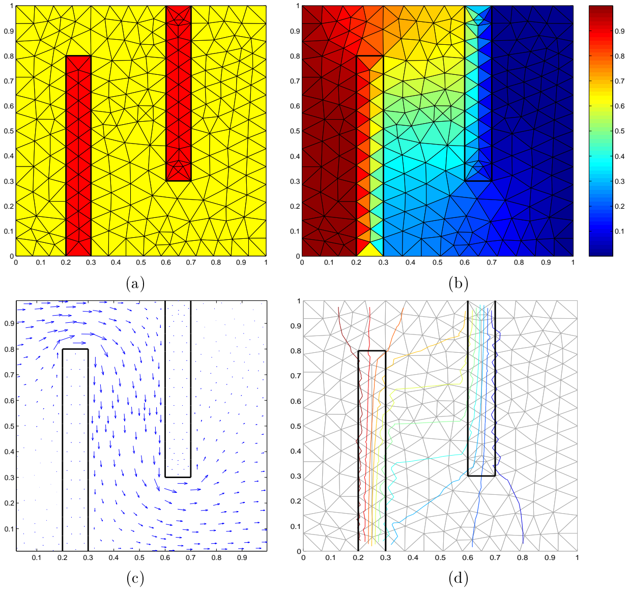
Figure 8: Fingers problem: (a) grid with material properties, (b) temperature distribution, (c) heat flux distribution, (d) temperature contour isolines
