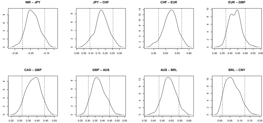
Figure 5.4: Estimated posterior densities of Kendall’s \tau in the crisis regime of Model (2a*) with 90% CIs. The plotted densities correspond to the parameters of the (unconditional) copulas associated to Tree 1 of the vine \mathcal{V}_2 .
