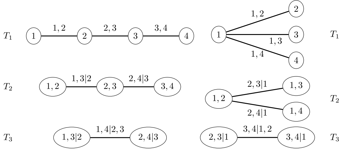
Figure 1.2: A D-vine (left panel) and C-vine (right panel) tree sequence in four dimensions.
