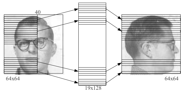
Fig. 2 MLP structure for synthesizing profiles.
