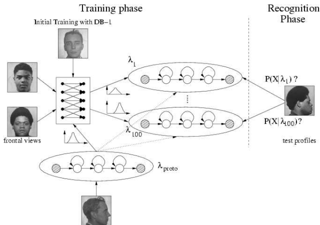
Fig. 5 Hybrid System consisting of a MLP and HMMs
