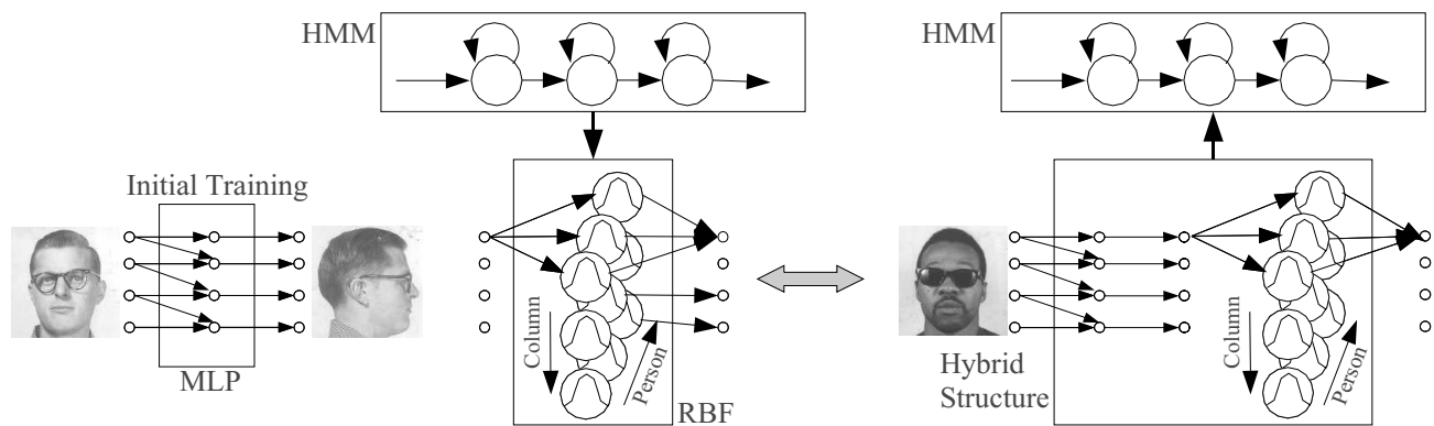
Fig. 7 Hybrid System consisting of a MLP, RBF/HMM
