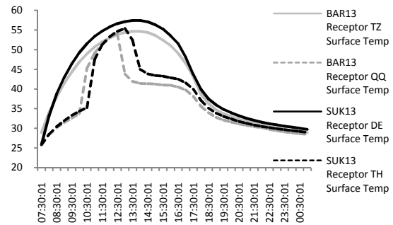
Figure 8: Surface temperature in Sukrabad and Baridharain
