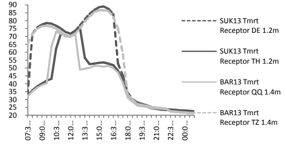
Figure 7: Comparison of MRT in Sukrabad and Baridharain
