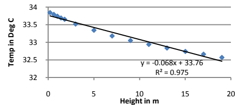
Figure 3: Temperature decreasing with height due to lapse rate
