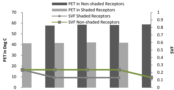
Figure 10: Comparison of PET value at 14:00 hours in shaded or non-shaded areas in Baridhara and Sukrabad
