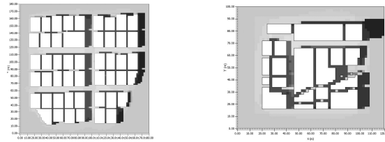
Figure 4: Comparison of MRT in Sukrabad and Baridharain N-S and E-W oriented streets
