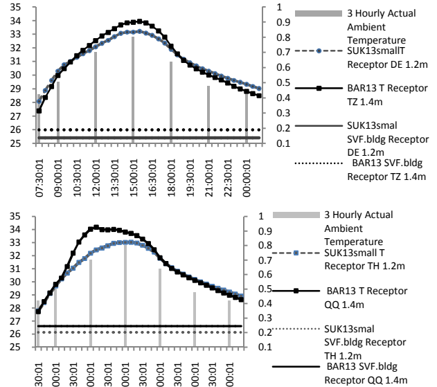
Figure 2: Comparison of Air Temp in Residential in E-W (a) and N-S(b) Street Canyons between Baridhara and Sukrabad
