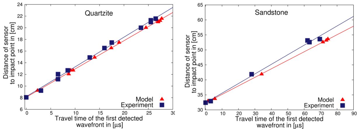
Fig. 11. Linear propagation of the first wave front inside the target for the experiment and the model. The plot shows the distances of different sensors dependent on the arrival time. The average wave velocity is measured to be around 5000 m/s (experiment) and 4900 m/s (model) for quartzite (left) and 3200 m/s (experiment) and 2900 m/s (model) for sandstone (right). Please note the different block sizes and thus scale on the x-axis. For the quartzite a 20-cm cubed target has been used, for the sandstone a 50-cm cubed target.
