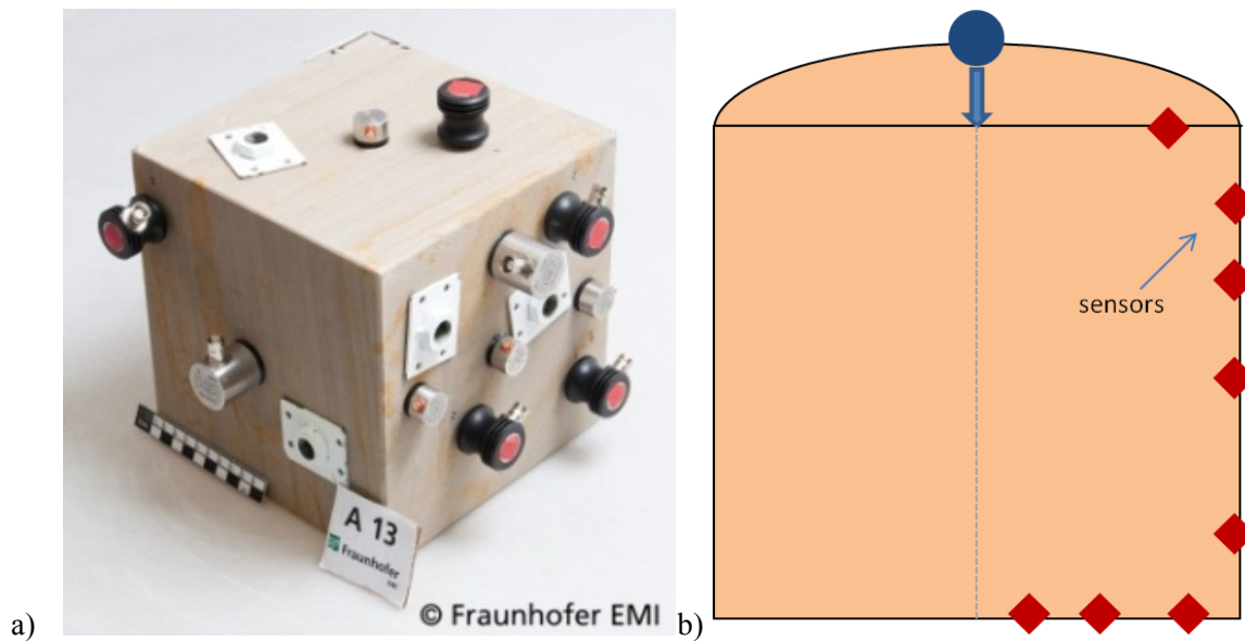
Fig. 1. Experimental and numerical setup. a) Setup of sensors and sandstone target for the AE experiment before the impact. b) Numerical setup of the target block with sensors. The numerical model uses a cylindrical target whereas the experimental target is represented by a cube.
