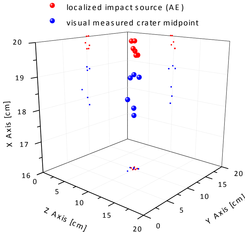
Fig. 8. Localization of six impact points of 20 cm cubed targets, respectively two sandstones, two quartzite, and two tuff targets. The red points show the localized impact points using AE data and the blue points represent the visually measured impact midpoints (bottom of the crater). The squares at the spatial sections are the projections of the impact points (all coordinates see Table 3).
