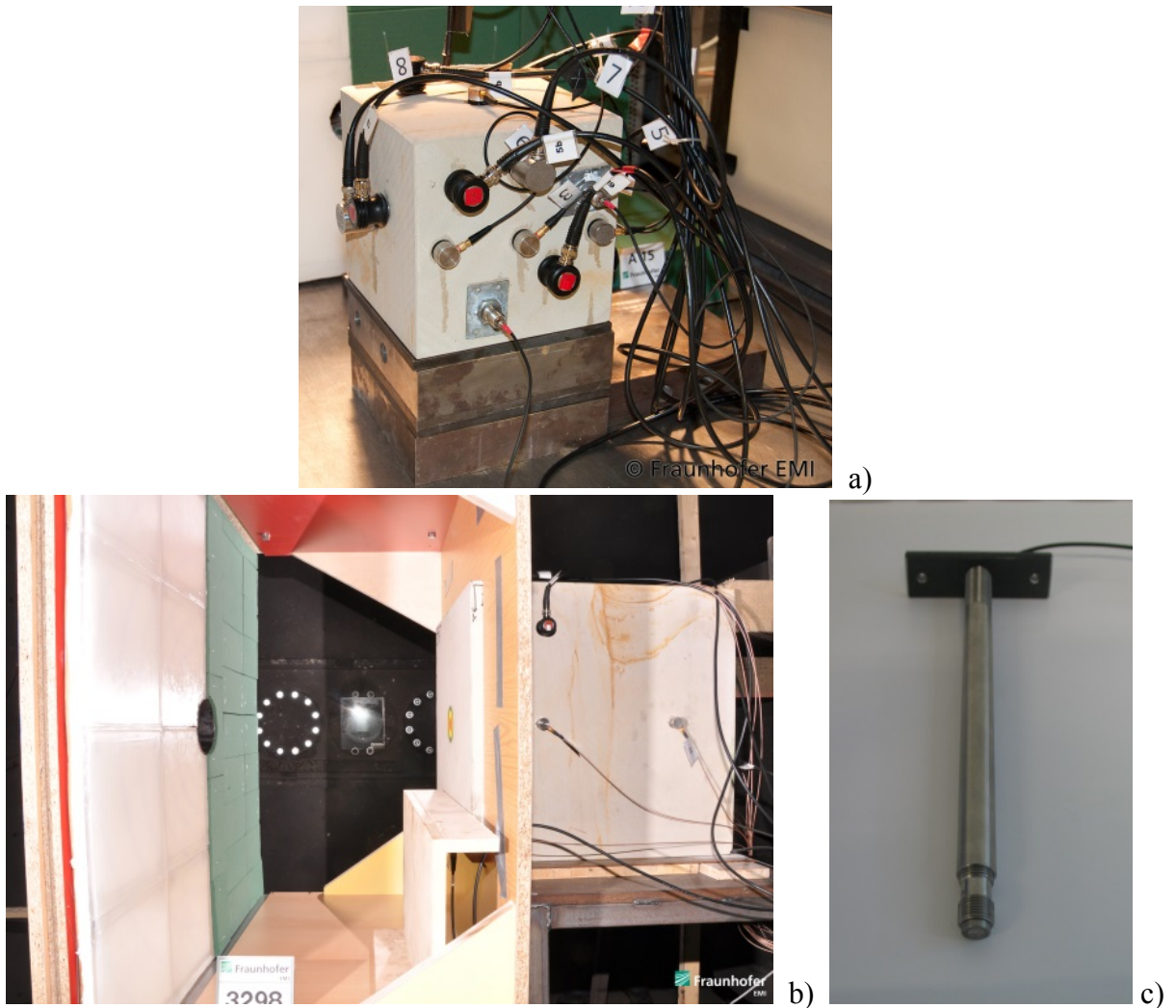
Fig. 5: a) Target (20 cm cubed) inside the chamber of the light gas gun, including the sensors for the AE measurements at the surface. b) Setup of the experiment inside the chamber, including the target with sensors on the right and the ejector catcher on the left. The target-surface was marked with concentric rings of different colors equipped with trace elements to reconstruct the origin of the ejected target material. c) Special sensor-holder with sensor for boreholes.
