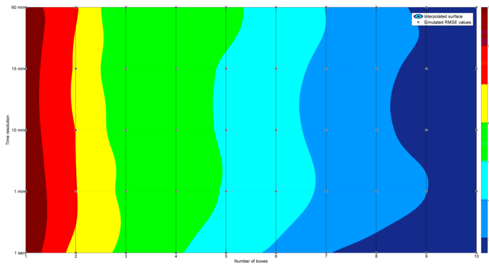
Figure 10: Contour plot of the root mean square error as a function of the number of measurement stations on the x-axis and the time resolution on the y-axis.
