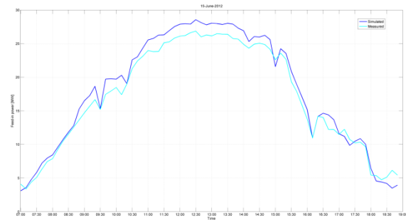
Figure 7: Comparison between the simulated (dark blue) and measured (light blue) feed-in power.
