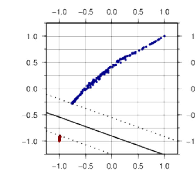
Figure 5: Example of a SVM model dividing two classes
