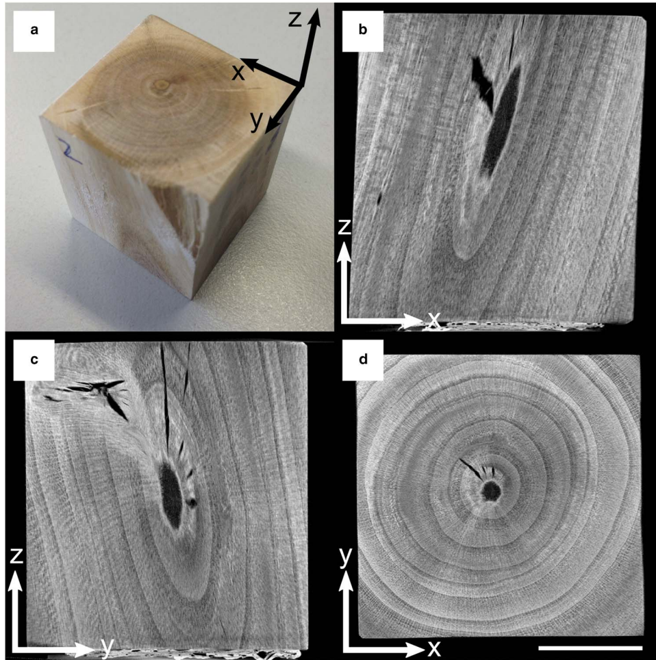
Figure 1. The wooden cube sample was cut out of a cherry tree branch. a: Photograph of the specimen demonstrating the chosen coordinate system. The cube had an edge length of 3 cm. b–d: Example micro-tomography slices through the cube volume showing the strong local orientation of the wood fibers. Scale bar is 1 cm.
