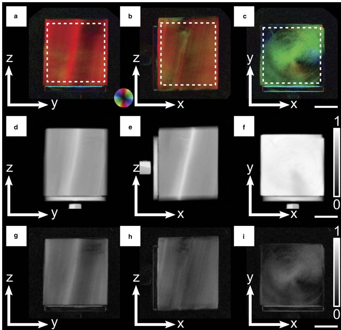
Figure 2. Visualization of the directional dark-field data of the wooden cube. The sample was mounted on a PMMA dish, which is visible as well. a–c: Dark-field X-ray radiographs showing orientation and anisotropy. The color specifies the local orientation, whereas the brightness encodes the local anisotropy. The orientation is extracted from the maxima/minima of the scattering signal. The anisotropy corresponds to the degree of fiber orientation. In (a) and (b) , the wood fibers are oriented approximately along the z direction; (c) shows the cube along the z axis, where it has a preferred orientation along the diagonal between the y and x directions. For a quantitative analysis, the average anisotropy and the average mean dark-field signal were calculated for all three orientations over the indicated areas. d–f: Mean dark-field projections giving the average scattering with respect to the rotation around the optical axis. The average scattering is related to the fiber density inside the specimen. g–i: Anisotropy images showing the anisotropy in the recorded scattering signal upon rotation. Scale bar is 1 cm.
