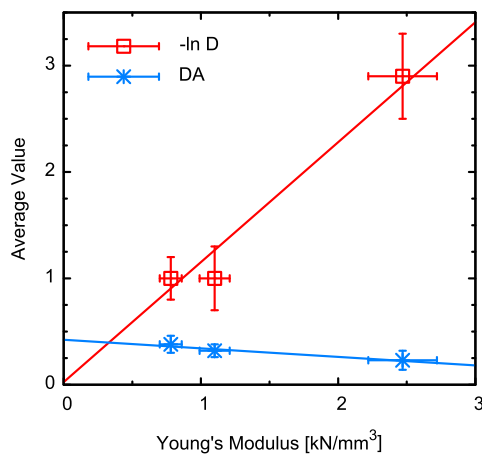
Figure 3. Plot of dark-field data against Young's modulus. The mean logarithmic dark-field signal -\ln D is shown in red, the anisotropy \overline{DA} in blue. Both quantities are correlated to the Young's modulus E . The average logarithmic dark-field signal is positively correlated ( R = 0.984 ) and the mean anisotropy shows a negative correlation ( R = -0.975 ) to the E modulus. The corresponding line fits are shown by dashed lines.
