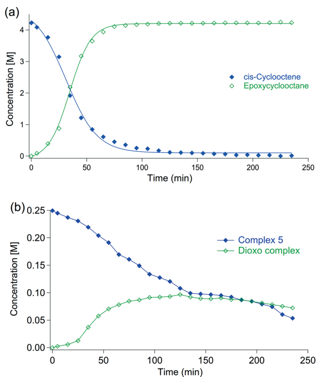
Fig. 7 Concentration vs. time plots for (a) catalytic epoxidation of cis -cyclooctene with TBHP and (b) the concentration of precatalyst 5 and the catalytically active oxidized complex (II) during epoxidation.
