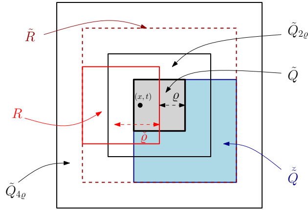
Figure 7.3: Illustrative example of spatial sides of the rectangles \tilde{Q} , \check{Q} , \tilde{Q}_{2\varrho} , \tilde{Q}_{4\varrho} , R , and \tilde{R}
