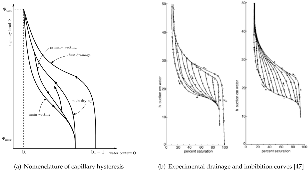
Figure 1.5: Capillary head - saturation relationship
