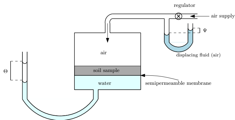
Figure 1.4: Experimental setup for measuring the capillary head in soil
