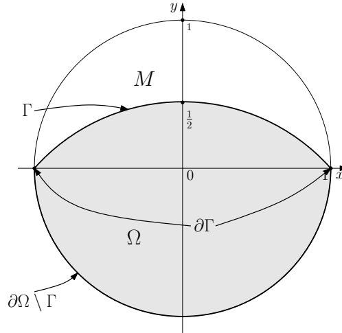
Figure A.1.1: Illustrative example of the special geometric density property
