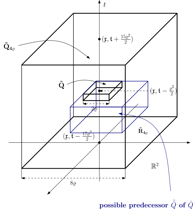
Figure 7.2: Illustrative example of the rectangles \tilde{Q} , \check{Q} , and \tilde{Q}_{4\varrho}
