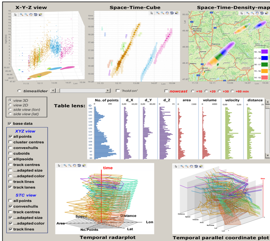
Figure 4. User interface of the visual analytical system for nowcasting of lightning behavior (Peters, 2014)
