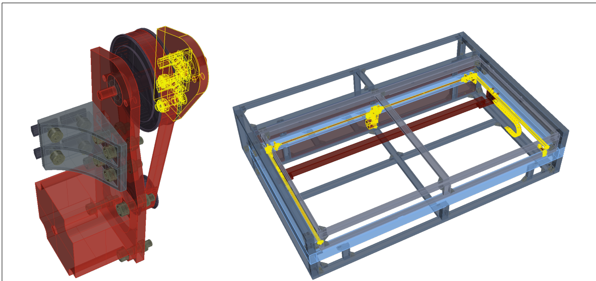
Image 4: CAD images from the Lasersaur manual; ( http://www.lasersaur.com/manual/build/6.y-drive.html , accessed 15.01.2015)
