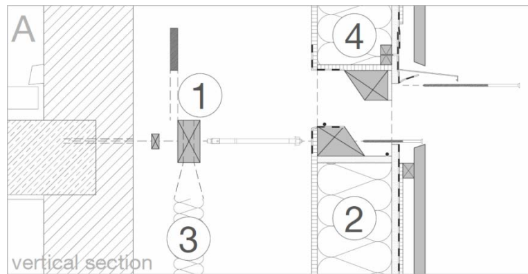
Figure 11: Mounting process
