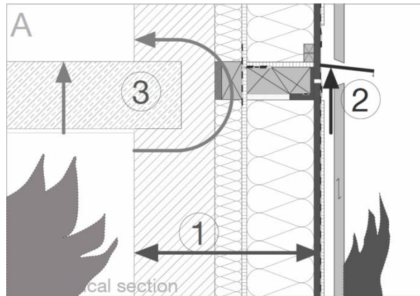
Figure 10: Fire safety detail
