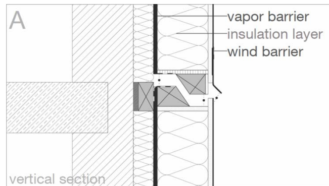
Figure 9: Hygrothermal Detail
