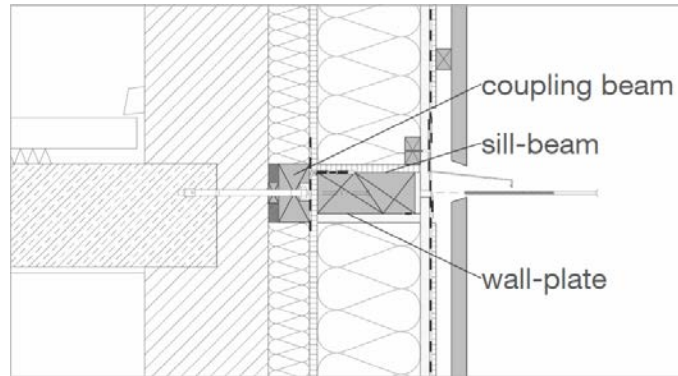
Figure 2: TES horizontal joint Vertical
