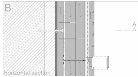
Figure 7: TES horizontal joint Horizontal
