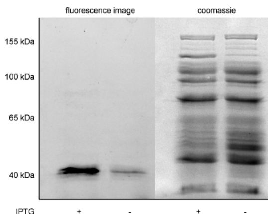
Fig. 3 Validation of protein target LipR. LipR was overexpressed in E. coli and labelled with lalistat probe La-1. Rhodamine-azide was attached via click reaction after cell lysis. The experiment was conducted with and without induction by IPTG (indicated with "+" and "-", respectively).
