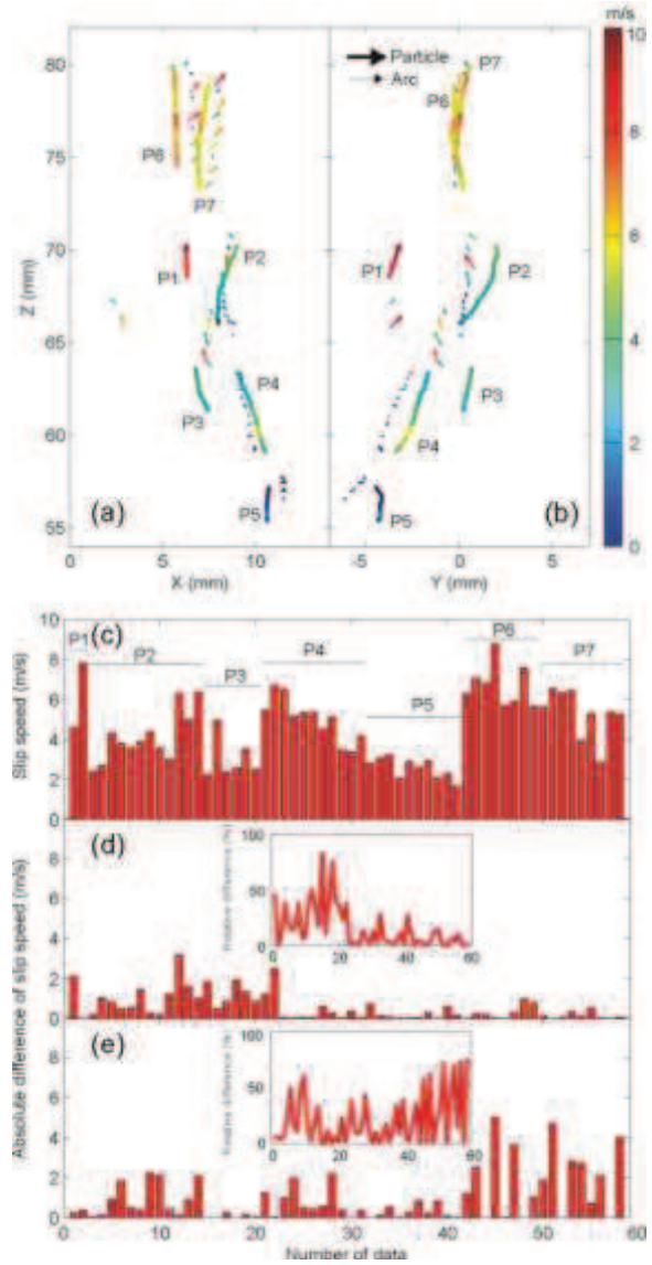
Fig. 4. Particle and plasma column velocity components in the (a) XZ and (b) YZ plane; (c) slip speed |\vec{V}_S| , V_S ; (d,e) absolute difference between the slip speed obtained by the 3D and the 2D method (the 2D method is performed for the (d) XZ and (e) YZ components). Relative differences (given in %) are inserted as subfigures. Particles P1-P7 are labeled in (a), (b), and (c).
