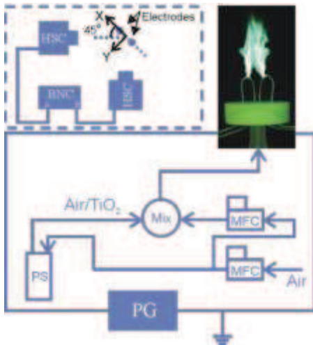
Fig. 1 Schematic of the experimental setup. HSC: high-speed camera; MFC: mass flow controller; PS: particle seeder; PG: power generator. The arrangement of the two cameras and the orientation of the electrodes are also illustrated.
