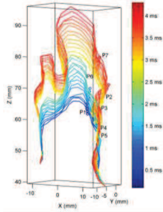
Fig. 3. 3D plasma column and particle reconstruction. Trajectories of seven seeding particles are marked (P1 to P7). The colors indicate the time evolution from 0 to 4 ms.
