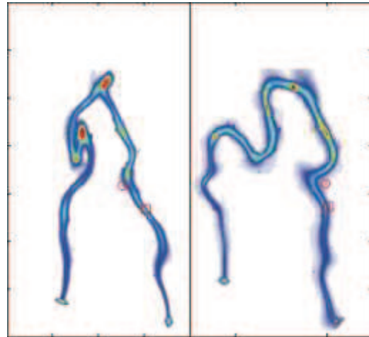
Fig. 2 An image pair of the gliding arc discharge simultaneously recorded by the two high-speed cameras. In this image, two typical seeding particles illuminated by the bright plasma column are highlighted by a red square and circle located on the right hand-side part of the plasma column.
