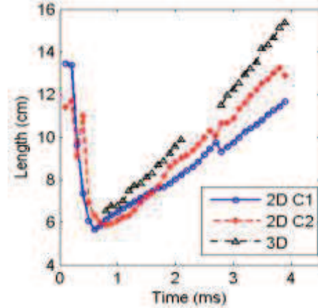
Fig.5 Length of the plasma column based on the 3D reconstruction and, respectively, the 2D camera images.
