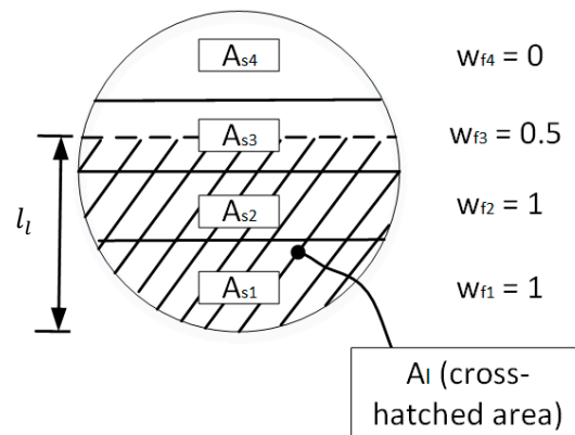
Figure A1. Cross-sectional areas and area fractions as a function of the liquid level (all areas here shown refer to only the cross-sectional area of the pipes).
