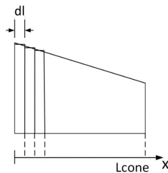
Figure A3. Discretization of the conic region.
