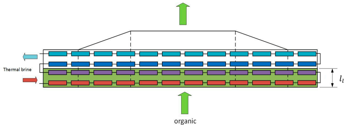
Figure 5. Kettle boiler side view and flow scheme.
