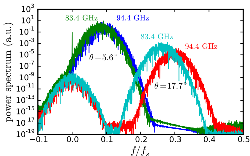
FIGURE B.1: Power spectra obtained from X-mode 2DFW simulations in linear regime. Two angles of incidence and two probing frequencies are presented.
